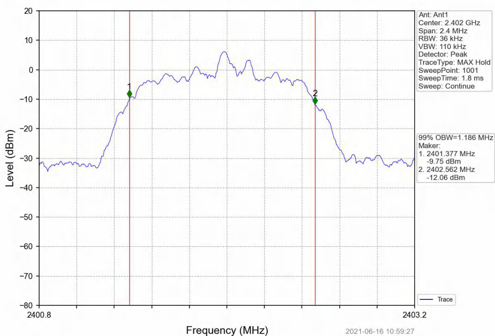
PI/4DQPSK_2DH5_LCH_2402MHz_Ant1_NTNV
