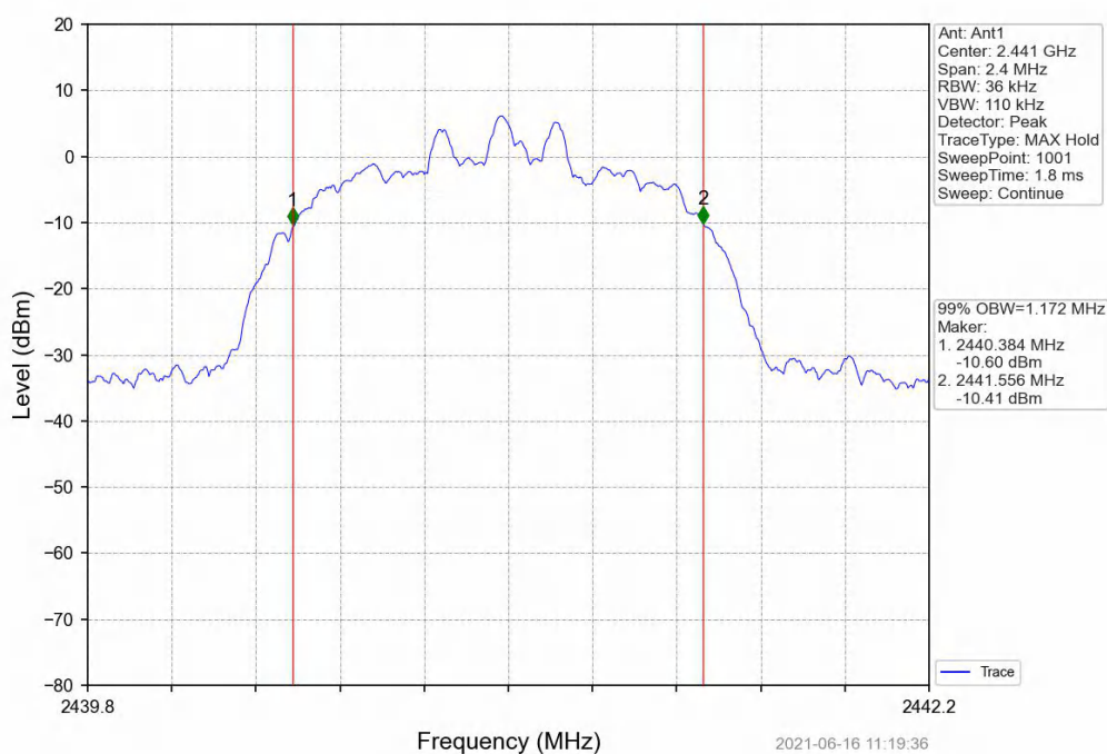
8DPSK_3DH5_MCH_2441MHz_Ant1_NTNV
