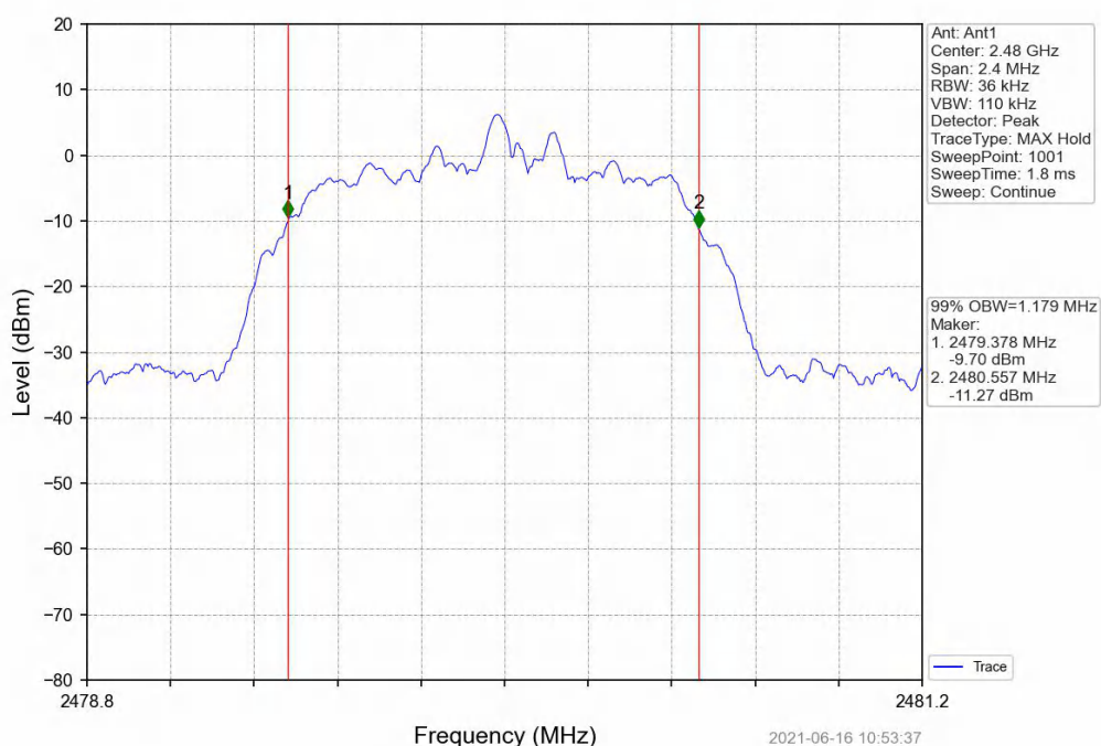
Pi/4DQPSK_2DH5_HCH_2480MHz_Ant1_NTNV
