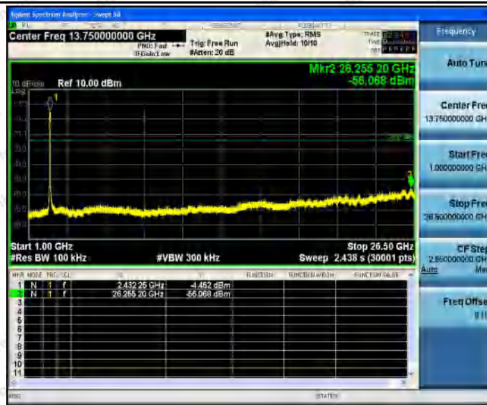
11N40_Ant2_2437_0~Reference
