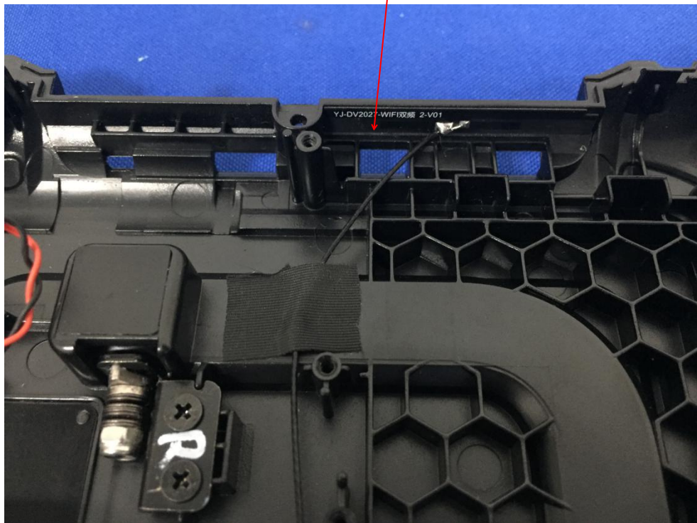
WIFI ANT 2
