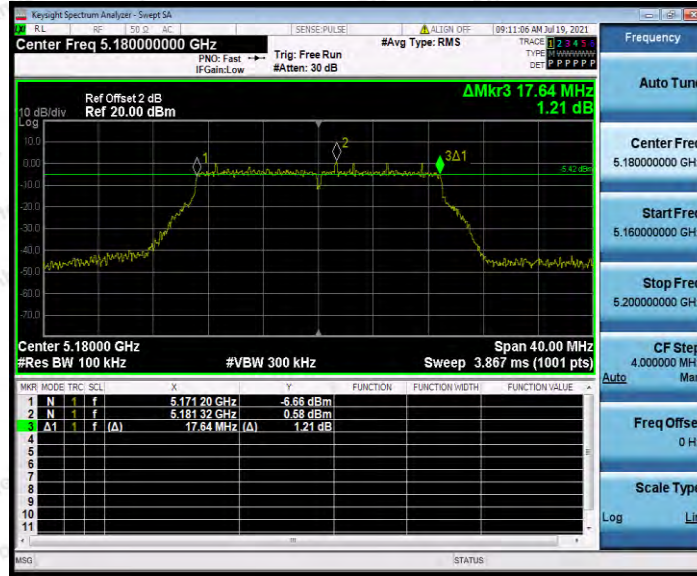
11AC20SISO_Ant2_5180
