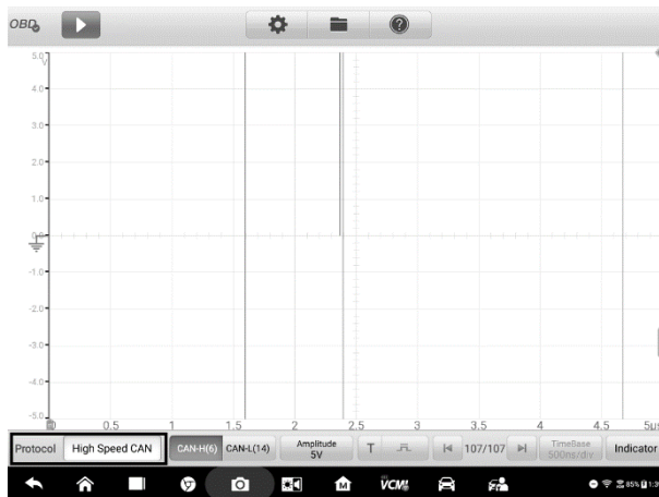
Figure 8-16 Sample Protocol Type Button Screen
