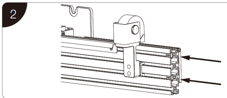
Figure 3-2 Insert Nuts
