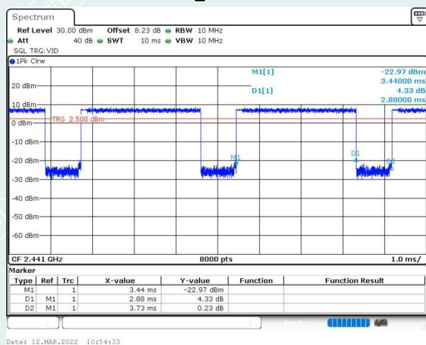
3DH5_2441MHz
