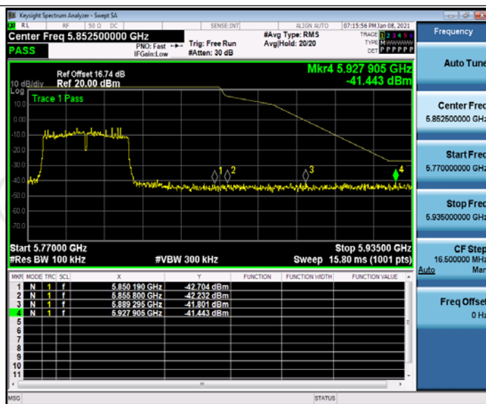
11AC40SISO_Ant1_High_5795
