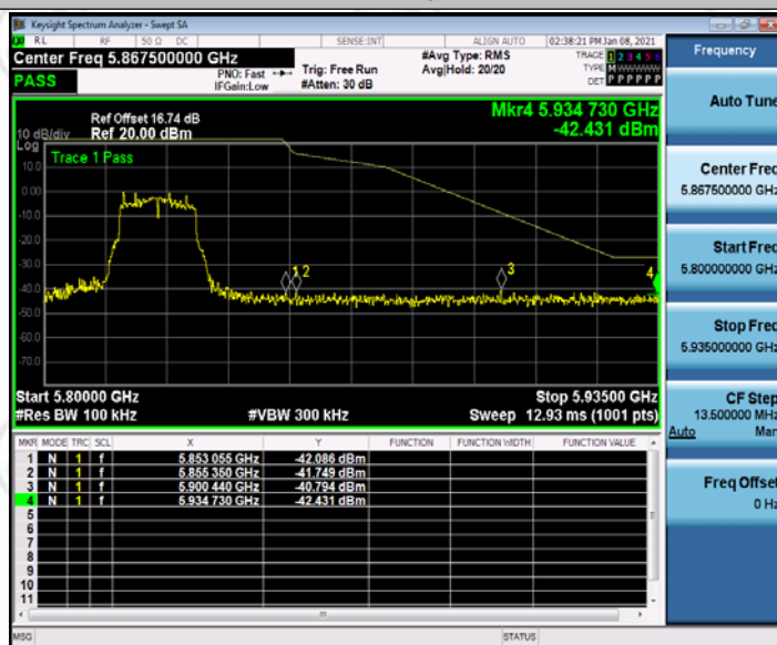
11A_Ant1_High_5825
