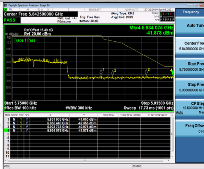
11AC80SISO_Ant1_High_5775
