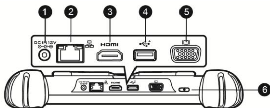
Figure 2-4 MaxiSys Tablet Top View
