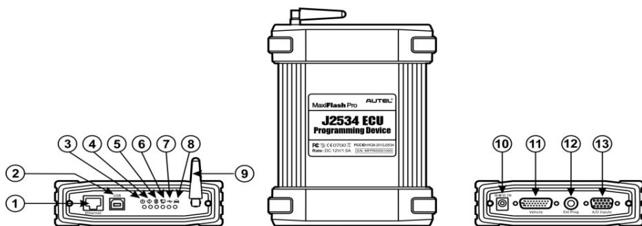
Figure 2-6 J2534 ECU Programming Device – for MaxiSys Pro
