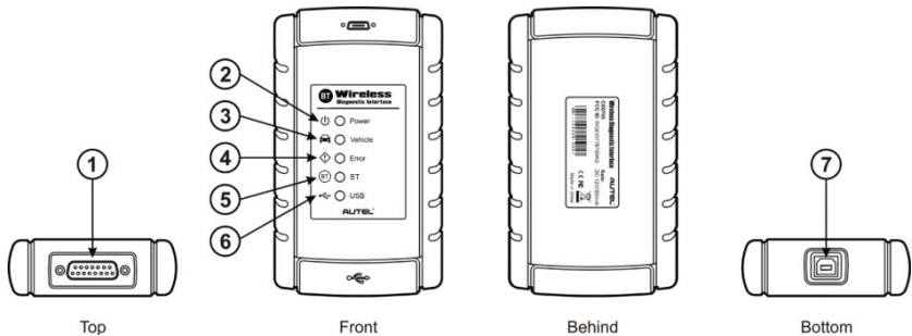
Figure 2-5 Wireless Diagnostic Interface – for MaxiSys
