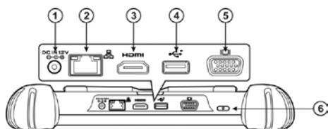
Figure 2-4 MaxiSys Tablet Top View
