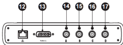
Figure 2-7 VCM Bottom View
