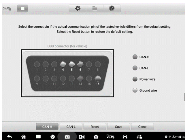
Figure 8-7 Sample Settings Menu Screen 3
