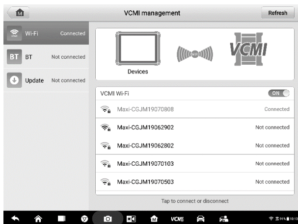
Figure 12-2 Sample Wi-Fi Connection Screen
