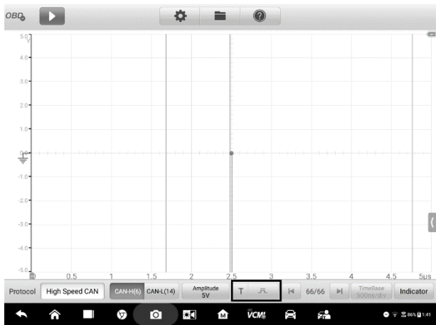
Figure 8-21 Sample Trigger Point Screen
