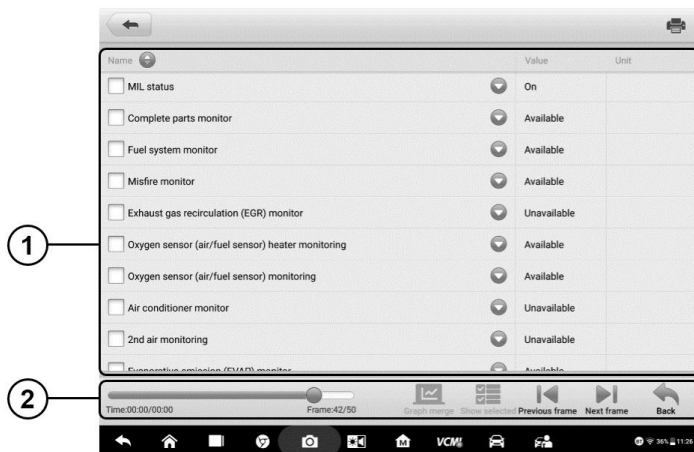
Figure 9-7 Sample Data Playback Screen
