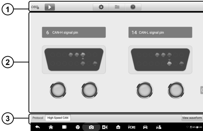
Figure 8-4 Sample OBD Communication Line Inspection Menu Screen
