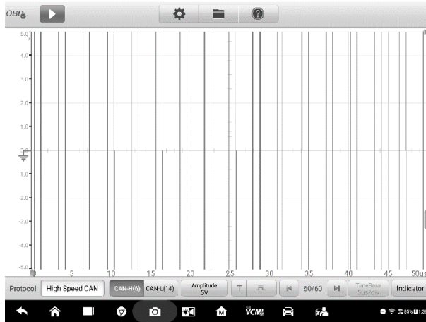
Figure 8-13 Sample Indicator Mode Screen
