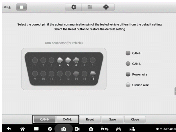
Figure 8-6 Sample Settings Menu Screen 2
