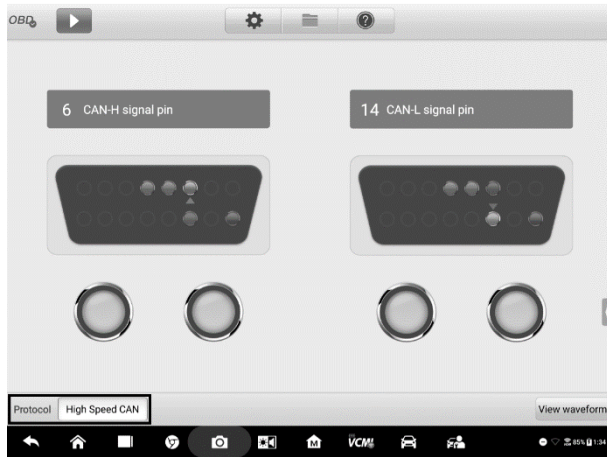
Figure 8-11 Sample Protocol Button Screen
