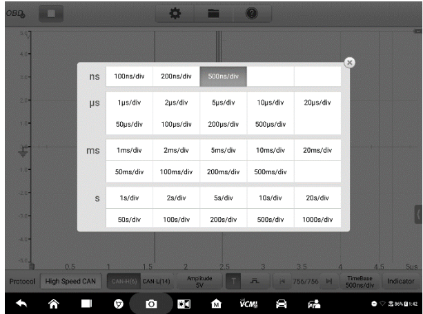
Figure 8-27 Sample Time Base Screen 2
