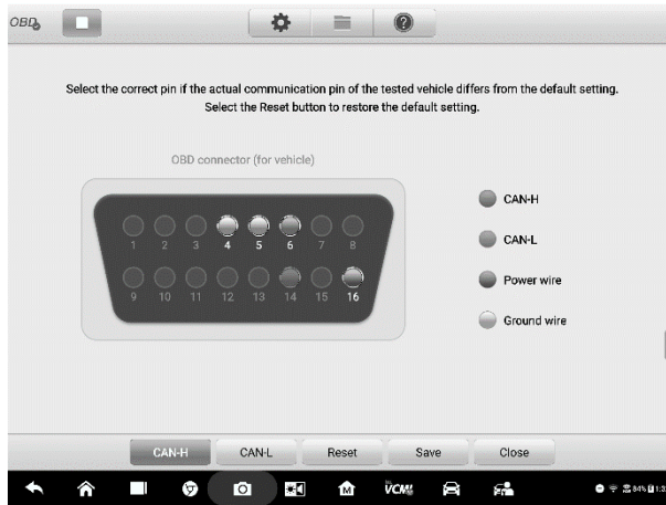
Figure 8-5 Sample Settings Menu Screen 1
