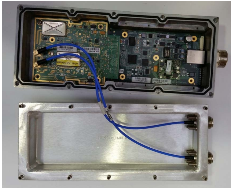
WIN5137-AC-IS - Internal view
