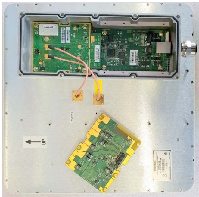
WIN5237 Internal view - Without PSU board
