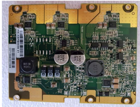
WIN5137-AC, WIN5137-DC, WIN5237 PSU board – Front view
