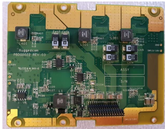
WIN5137-AC, WIN5137-DC, WIN5237 PSU board – Rear view
