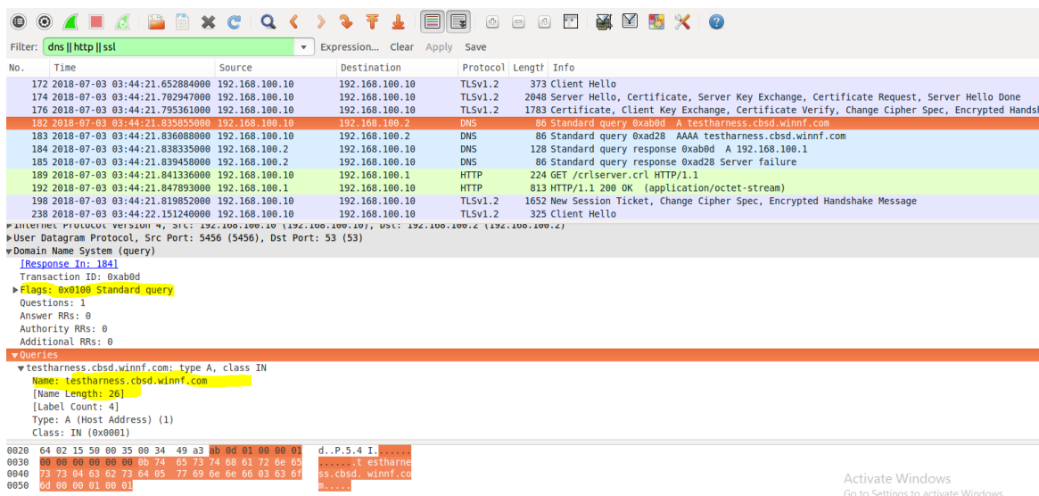
Figure 9.30-1: DNS
