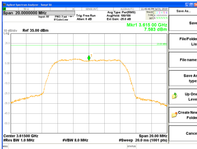
Figure 8.35-5: Base station frequency = 3615 MHz
