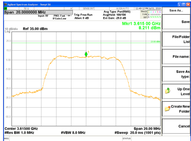
Figure 8.35-6: CPE frequency = 3615 MHz
