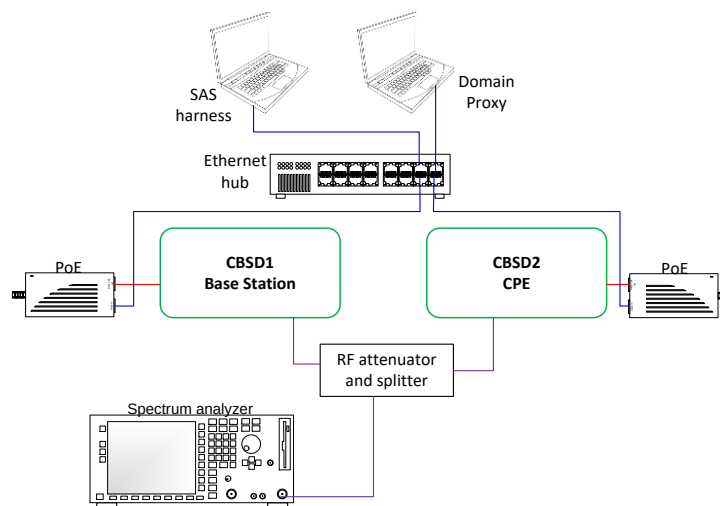
Figure 3.6-1: Setup diagram
