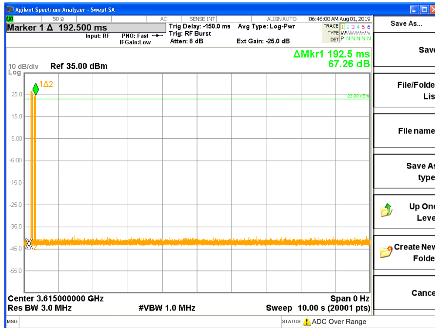
Figure 8.35-2: Time should not exceed 1 second within any 10-second period
