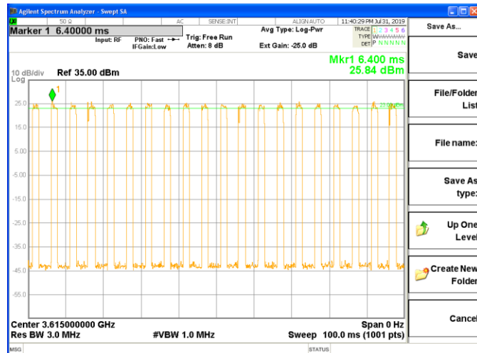
Figure 8.35-8: Power above 23 dBm, without ant gain
