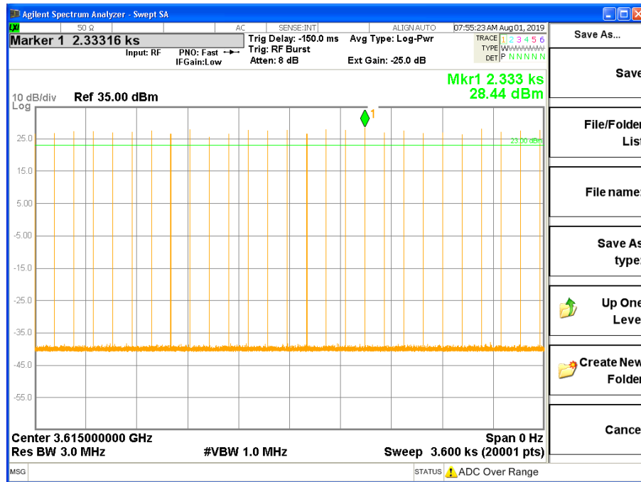
Figure 8.35-4: Time should not exceed 20seconds within any 3600-second period
