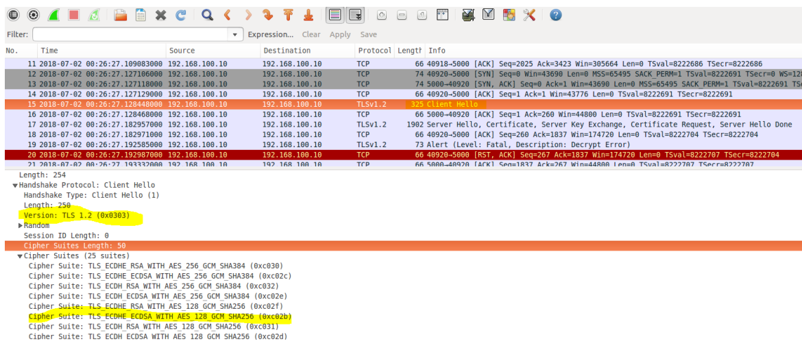
Figure 9.33-1: Client hello
