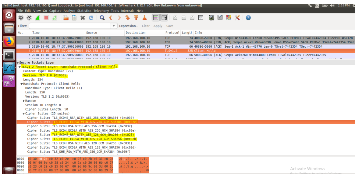
Figure 9.29-1: Client hello
