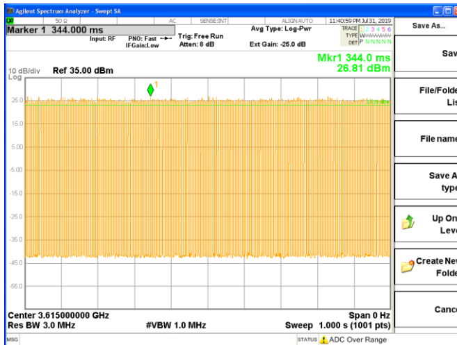
Figure 8.35-7: Power above 23 dBm, without ant gain
