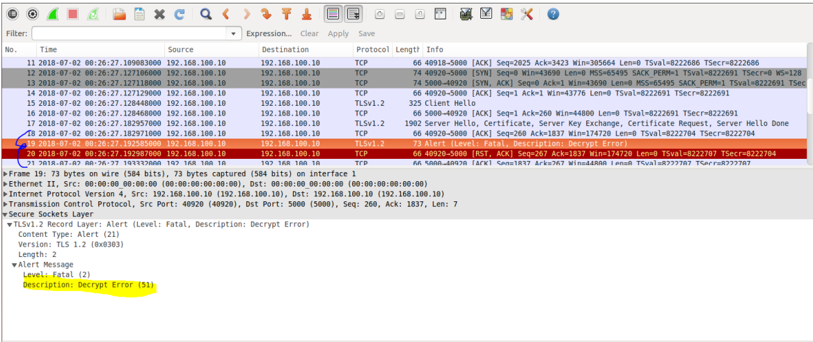
Figure 9.33-2: Close connection
