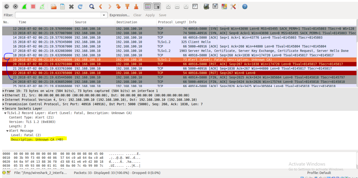
Figure 9.32-2: Close connection
