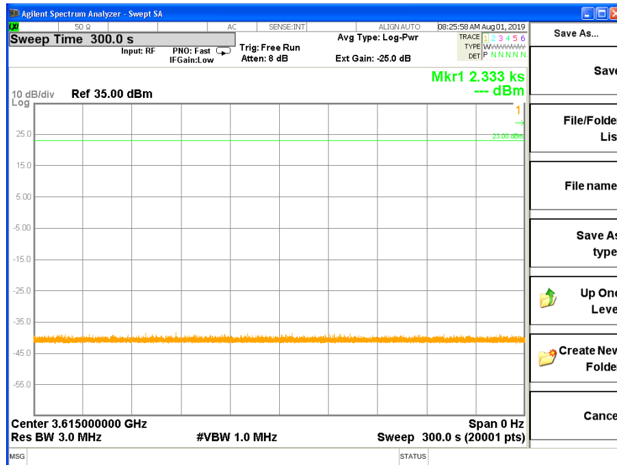
Figure 8.35-1: CPE-CBSD as UUT does not transmit
