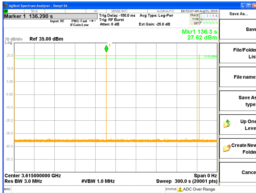
Figure 8.35-3: Time should not exceed 10seconds within any 300-second period
