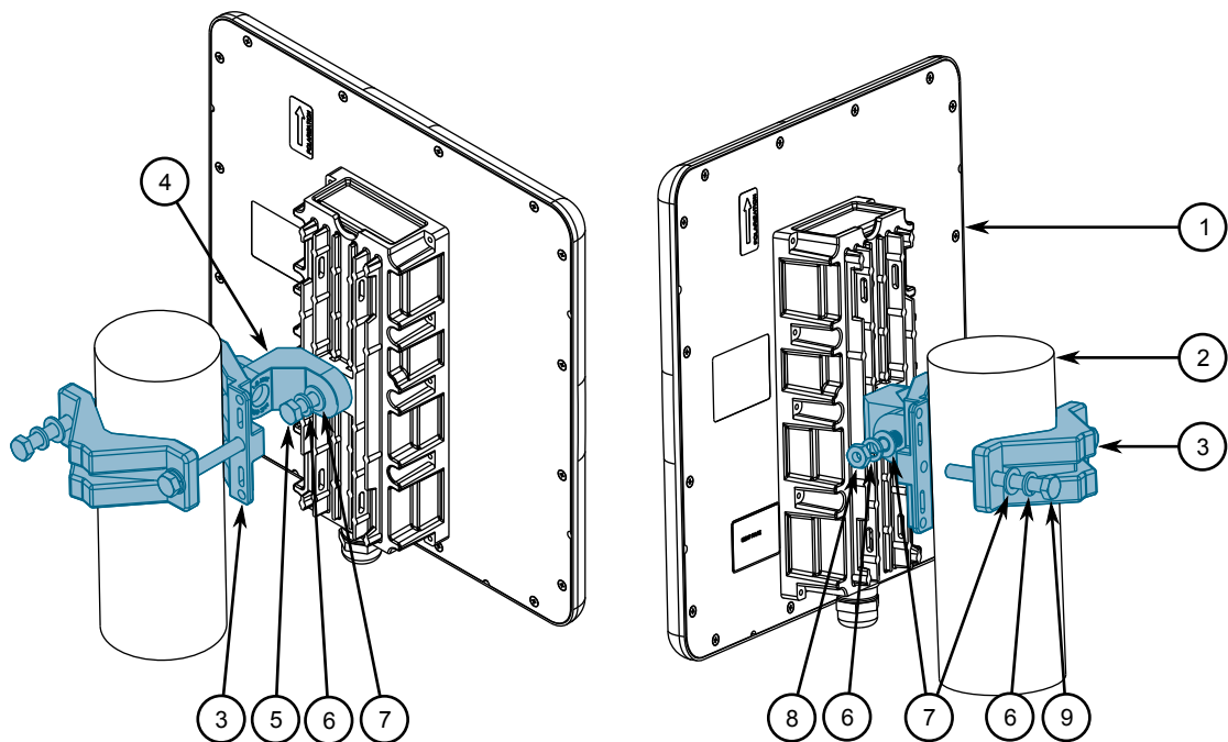
Figure 4: Mounting the Subscriber Unit to a Large Pole
