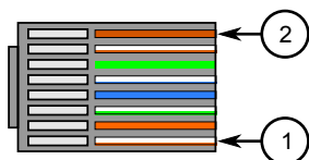
Figure 12: CAT-5e PoE Cable Pin-Out
