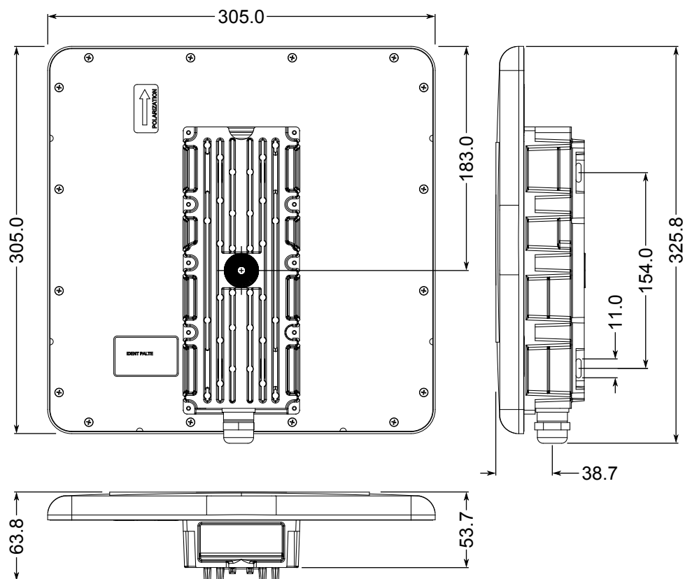
Figure 15: Overall Dimensions
