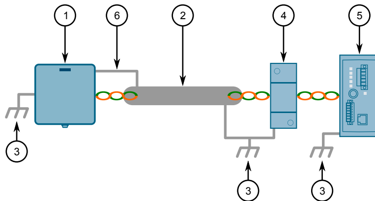
Figure 6: Typical Outdoor Installation
