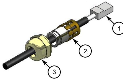
Figure 14: Assembling the Connector Components
