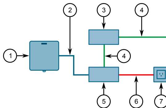
Figure 5: Connecting the RUGGEDCOM WIN1010 PoE Injector
