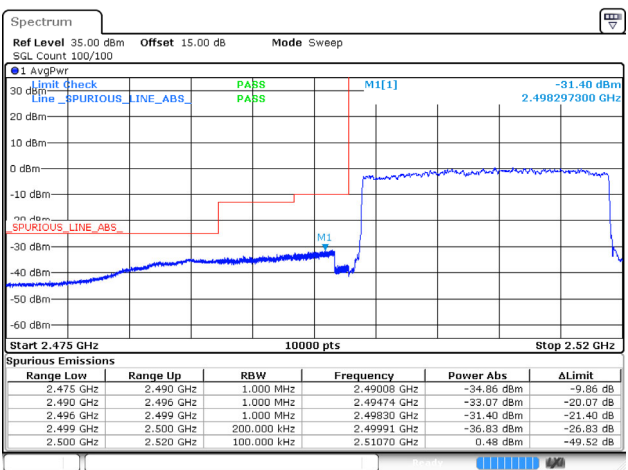
20MHz_Low_16QAM_100@0
