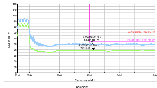
802.11n HT20-Channel 48: Peak + Average
