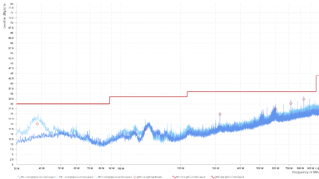
Radiates Emission from 30MHz to 1GHz
