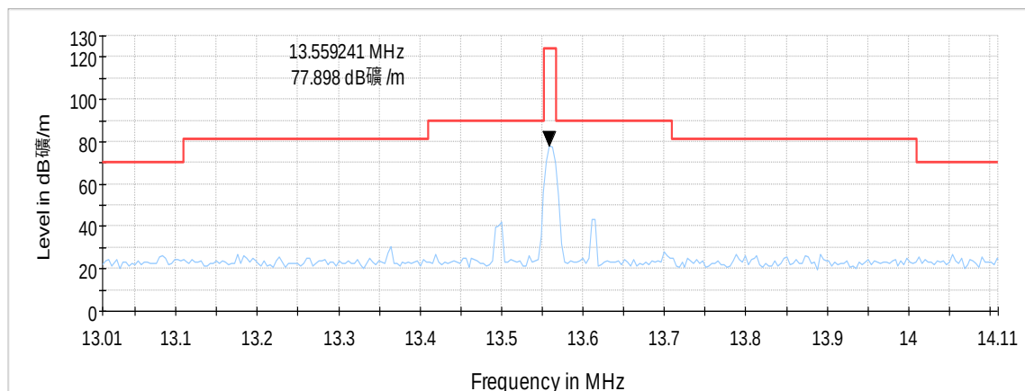
Radiates Emission from 13.01MHz to 14.11MHz
