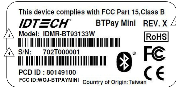
Box LABEL PRINTING DETAIL
