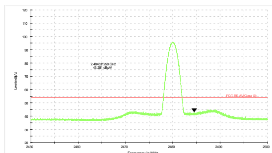
DH5-Channel 78: Average
