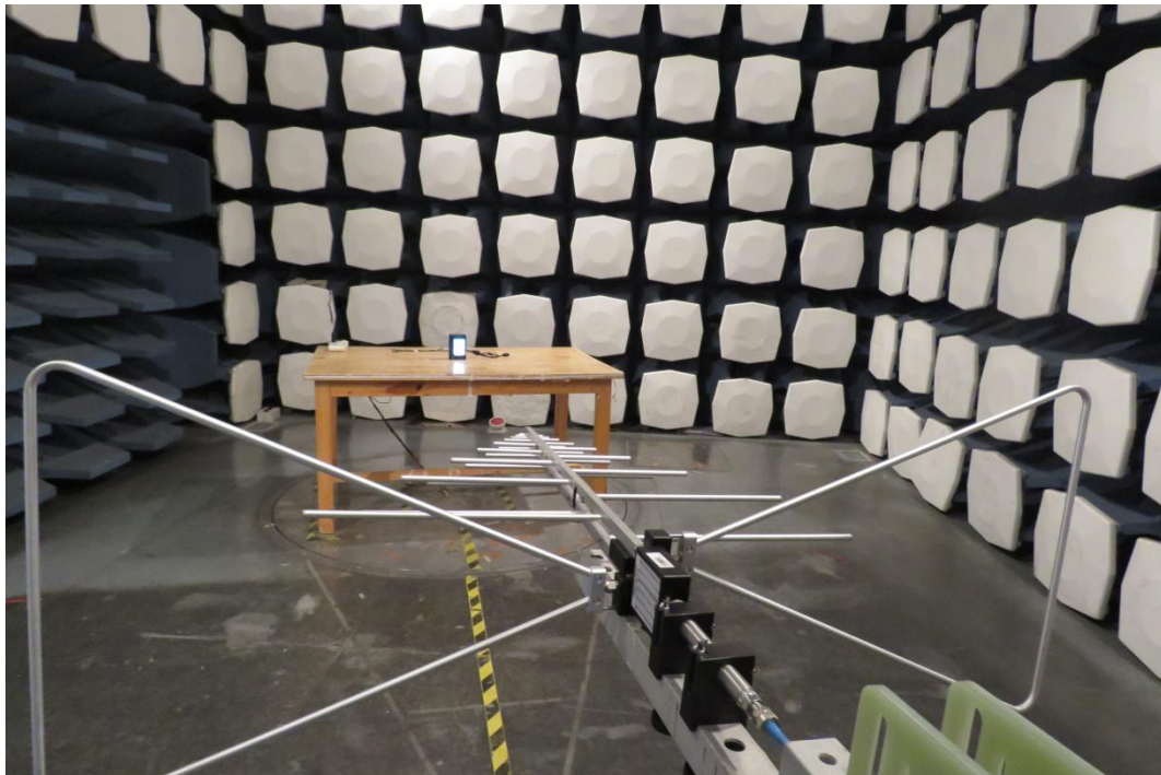
Below 1GHz
