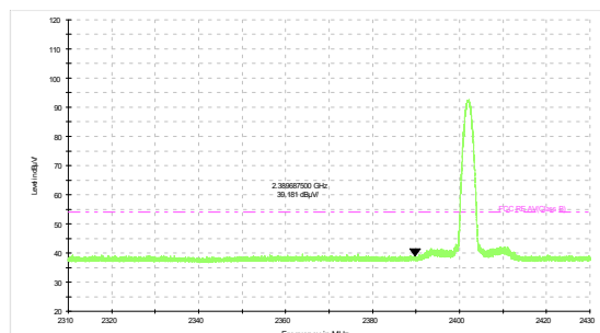
DH5-Channel 0: Average
