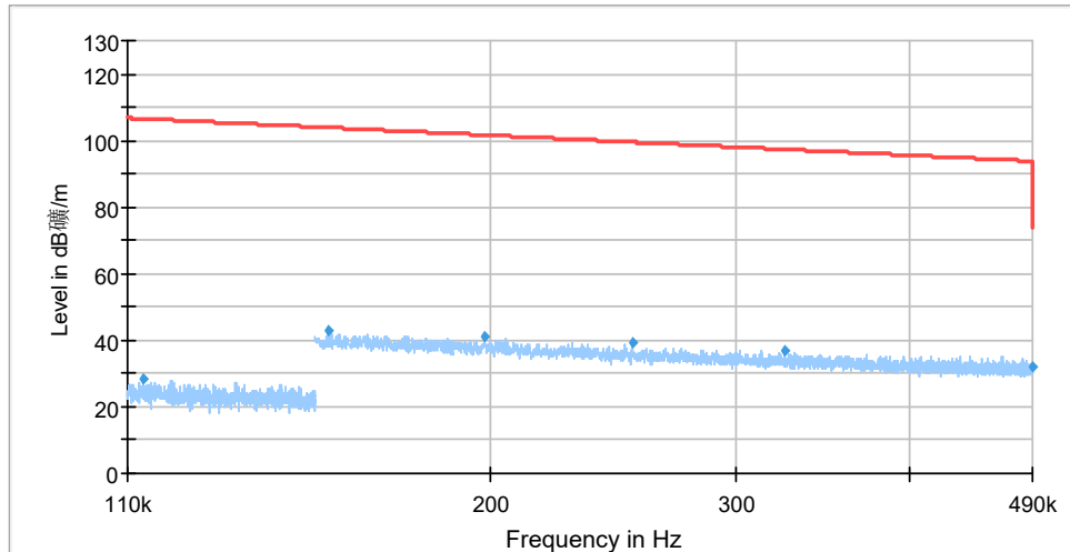
Radiates Emission from 110kHz to 490kHz
