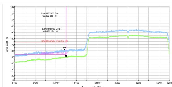
802.11ac VHT80 –Channel 42: Peak + Average
