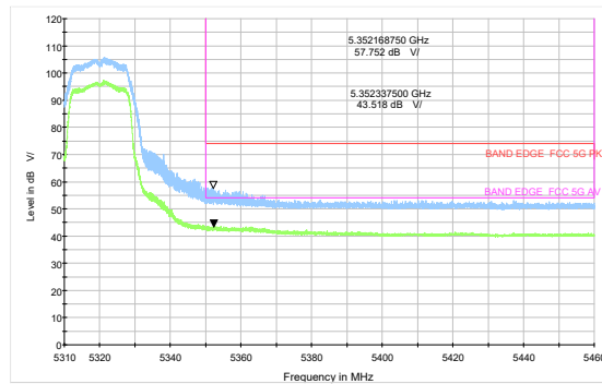
802.11n HT20-Channel 64: Peak + Average
