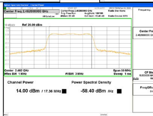
SDM Mode_802.11n_HT20_ANT1
