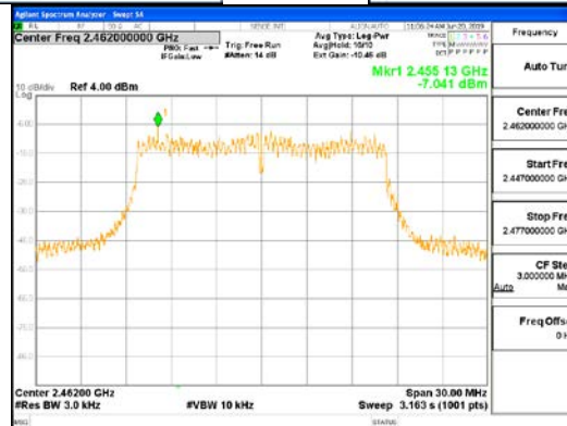
CDD Mode_802.11g_ANT2
