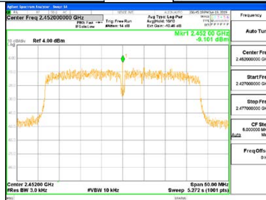
SDM Mode_802.11n_HT40_ANT2
