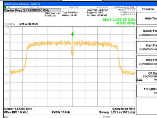
CDD Mode_802.11n_HT40_ANT2
