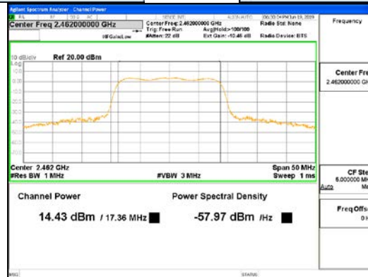
SDM Mode_802.11n_HT20_ANT2
