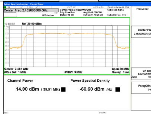
SDM Mode_802.11n_HT40_ANT1
