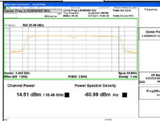
CDD Mode_802.11n_HT40_ANT1
