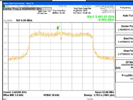
CDD Mode_802.11n_HT20_ANT2
