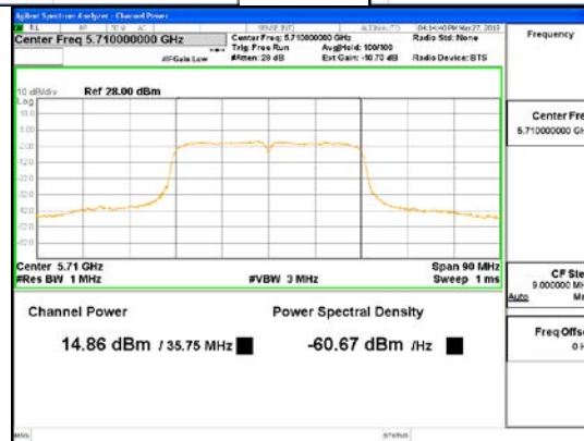
SDM Mode_ANT1_802.11n_HT40_UNII 2C
