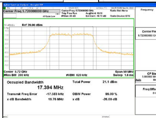
ANT3_802.11n_HT20_UNII 2C
