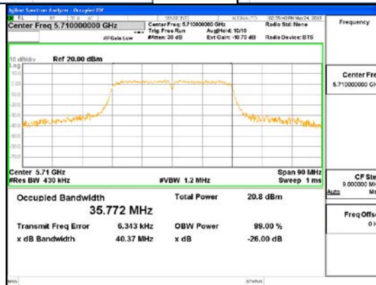
ANT2_802.11n_HT40_UNII 2C
