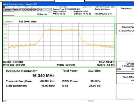
ANT3_802.11a_UNII 2C
