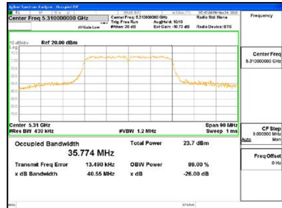
ANT3_802.11ac_VHT40_UNII 2A
