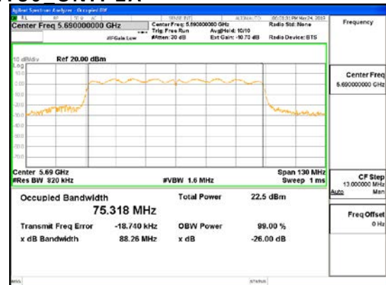
ANT3_802.11ac_VHT80_UNII 2C
