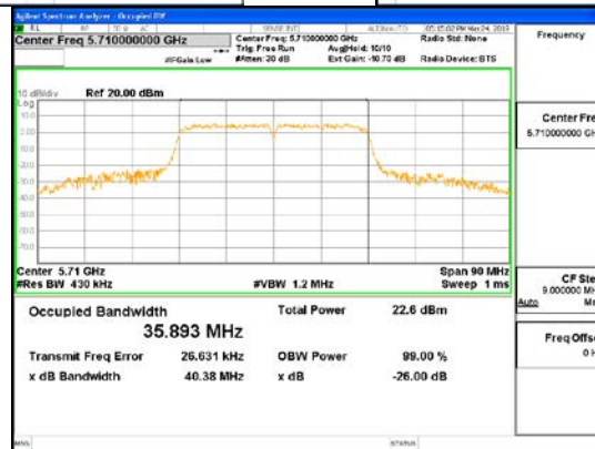
ANT3_802.11n_HT40_UNII 2C
