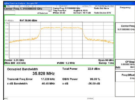
ANT2_802.11n_HT40_UNII 2A
