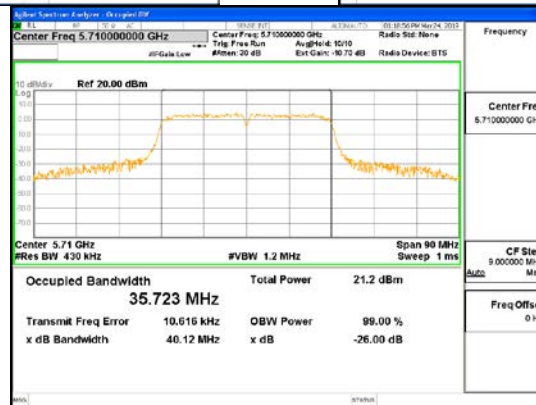
ANT1_802.11n_HT40_UNI1 2C
