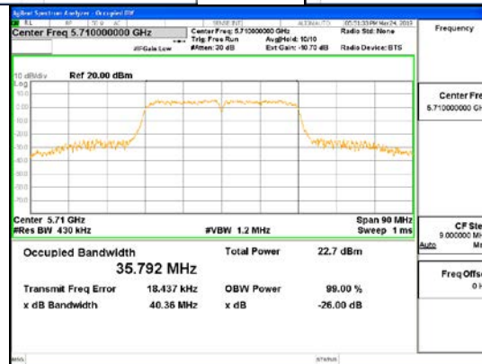
ANT3_802.11ac_VHT40_UNII 2C
