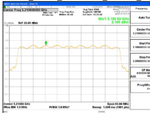
CDD Mode_ANT2_802.11ac_VHT80_UNII-1
