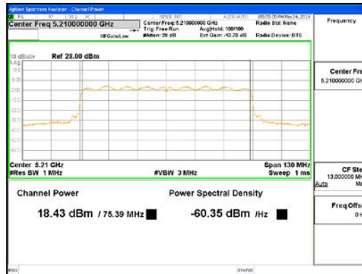
CDD Mode_ANT3_802.11ac_VHT80_UNII-1
