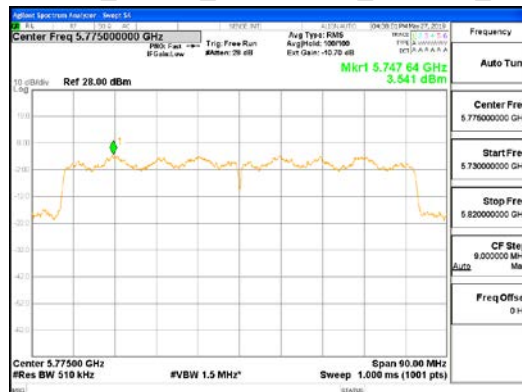
SDM Mode_ANT2_802.11ac_VHT80_UNII-3
