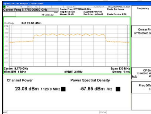
CDD Mode_ANT3_802.11ac_VHT80_UNII-3
