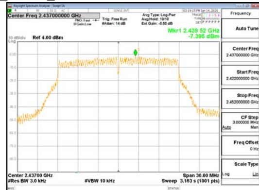
SDM Mode_802.11n_HT20_ANT1
