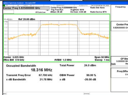
ANT4_802.11ac_VHT20_UNII-3
