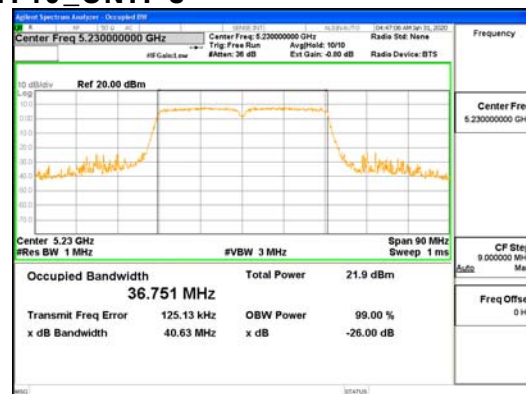
ANT2_802.11ac_VHT40_UNII-1
