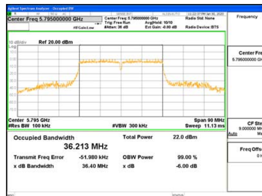
ANT1_802.11n_HT40
