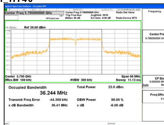
ANT2_802.11n_HT40
