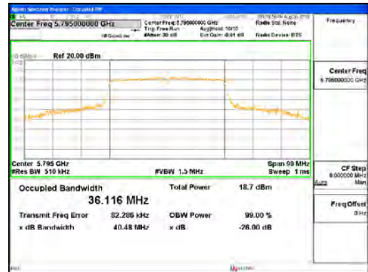
ANT0_802.11ac_VHT40_UNII 3
