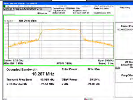
ANT0_802.11ac_VHT20_UNII 2A
