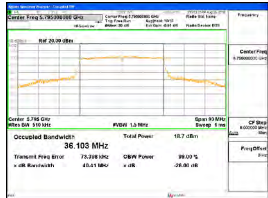
ANT0_802.11n_HT40_UNII 3
