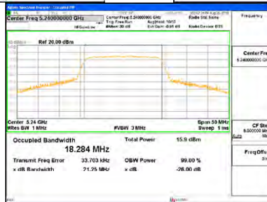
ANT1_802.11n_HT20_UNI1 1
