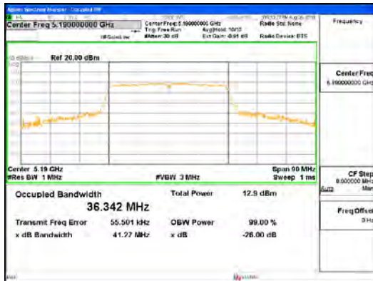
ANT0_802.11ac_VHT40_UNII 1
