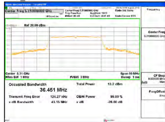
ANT0_802.11ac_VHT40_UNII 2A
