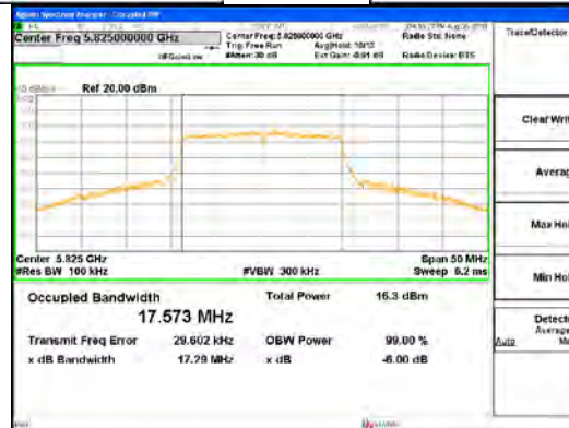
ANT1_802.11ac_VHT20
