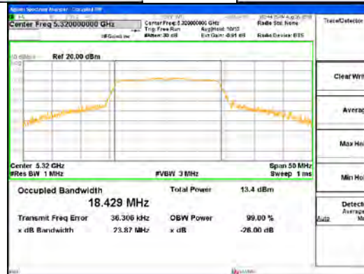
ANT0_802.11n_HT20_UNI1 2A
