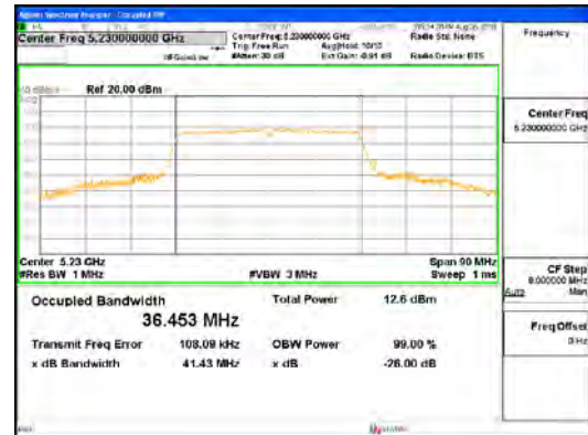
ANT0_802.11ac_VHT40_UNII 1
