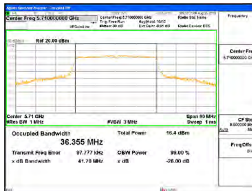
ANT0_802.11ac_VHT40_UNII 2C
