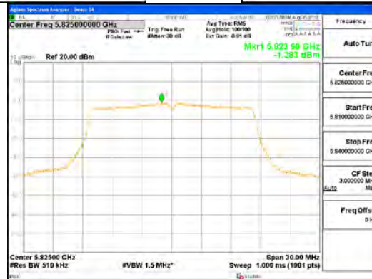
ANT0_802.11a_UNII 3
