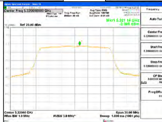
ANT0_802.11a_UNII 2A
