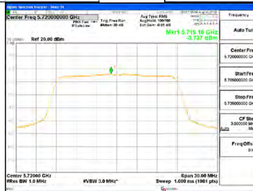
ANT1_802.11ac_VHT20_UNII 2C
