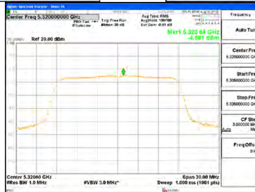
ANT0_802.11ac_VHT20_UNII 2A
