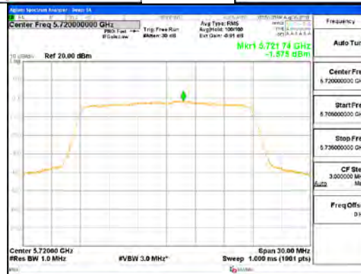
ANT0_802.11n_HT20_UNII 2C
