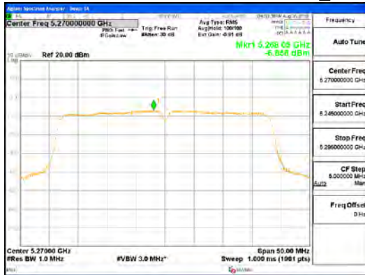
ANT0_802.11n_HT40_UNII 2A
