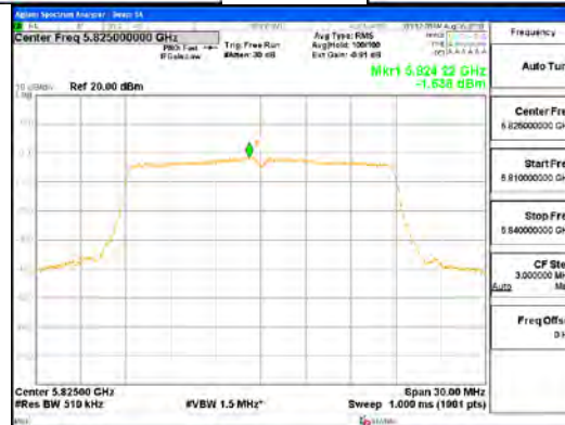
ANT0_802.11n_HT20_UNII 3
