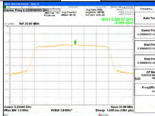
ANT0_802.11n_HT20_UNII 2A
