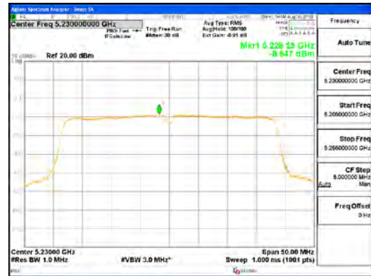
ANT0_802.11n_HT40_UNII 1
