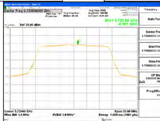
ANT0_802.11a_UNII 2C
