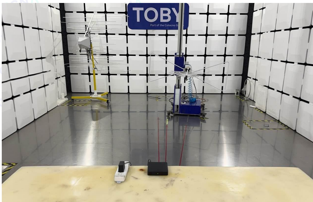
Photo of Setup for Radiated Emission (30MHz~1GHz)
