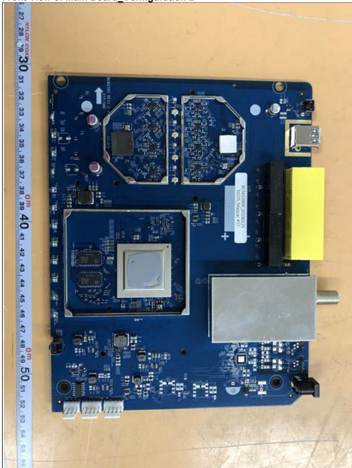
Front View of Main Board_Configuration 2
