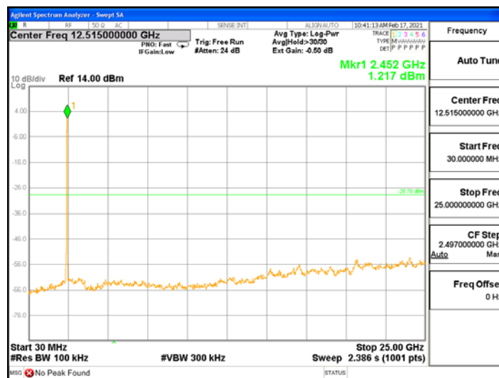
ANT4, 802.11n_HT40
