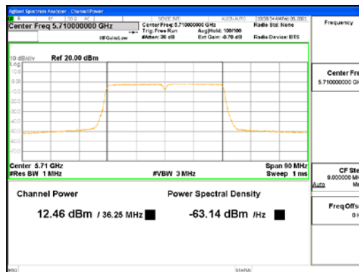
ANT4_802.11ac_VHT40_UNI1 2C
