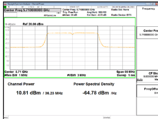
ANT3_802.11n_HT40_UNII 2C
