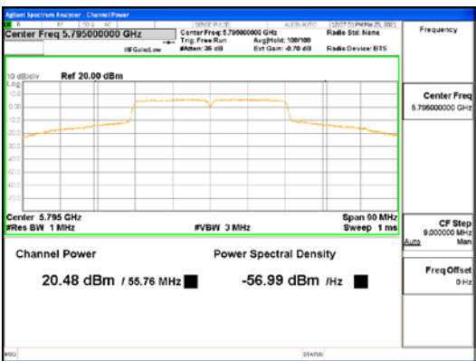
ANT4_802.11n_HT40_UNII 3
