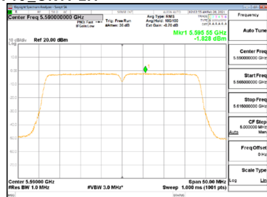
ANT3_802.11ac_VHT40_UNII 2C
