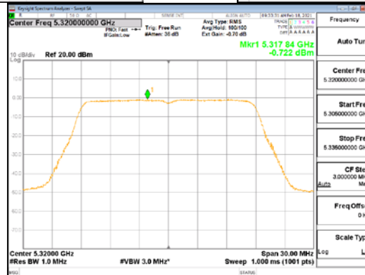
ANT3_802.11ac_VHT20_UNII 2A
