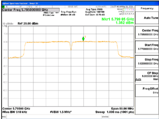
ANT3_802.11n_HT40_UNII 3
