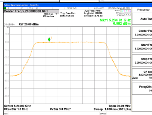
ANT4_802.11ac_VHT20_UNII 1
