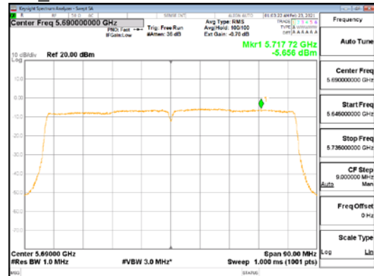
ANT3_802.11ac_VHT80_UNII 2C
