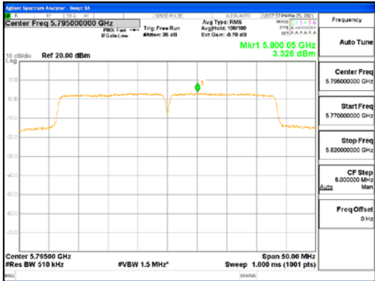
ANT4_802.11n_HT40_UNII 3
