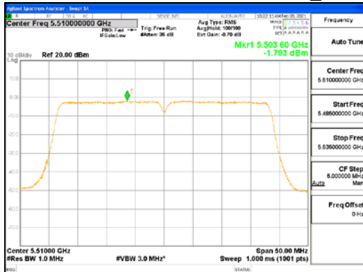
ANT2_802.11n_HT40_UNII 2A
