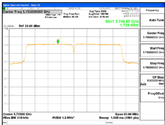
ANT2_802.11n_HT40_UNII 3
