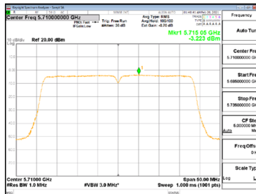
ANT3_802.11n_HT40_UNII 2C
