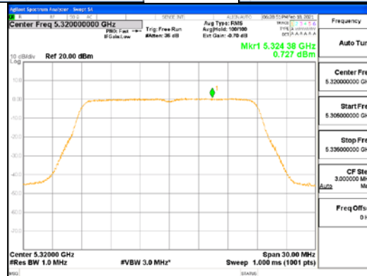
ANT4_802.11ac_VHT20_UNII 2A
