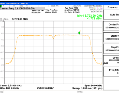
ANT4_802.11ac_VHT40_UNII 2C
