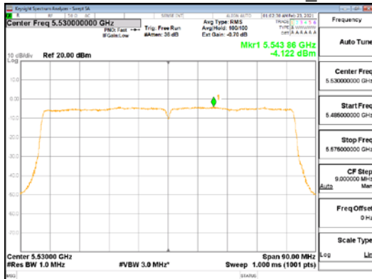
ANT3_802.11ac_VHT80_UNII 2C
