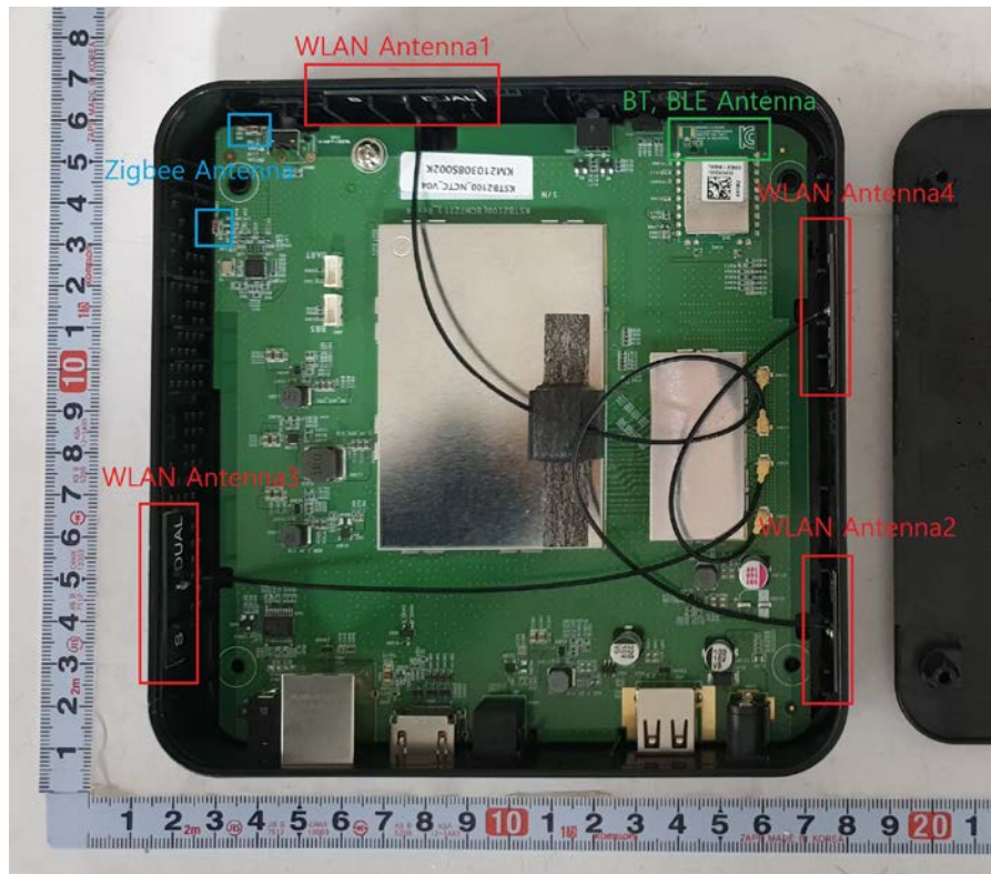
[WLAN_Antenna1]
