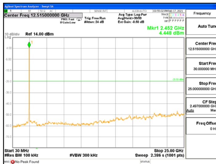
ANT4, 802.11n_HT20
