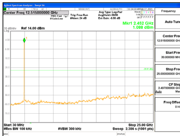
ANT2, 802.11n_HT40
