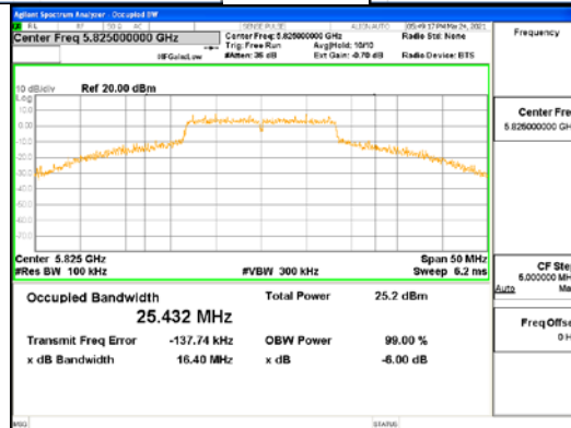
ANT4_802.11a
