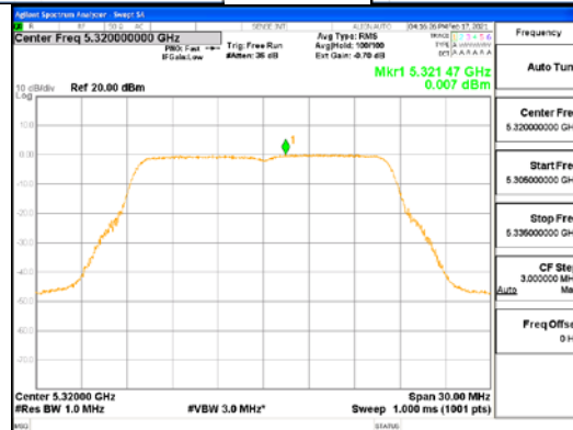
ANT2_802.11a_UNII 2A
