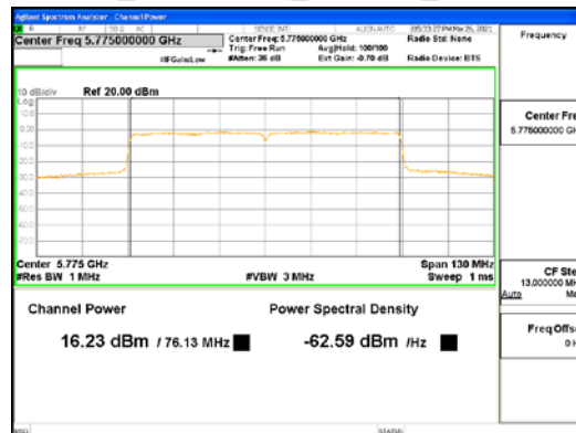
ANT1_802.11ac_VHT80_UNII 3
