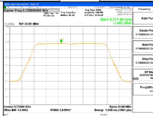
ANT4_802.11n_HT20_UNII 2C
