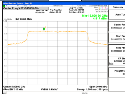
ANT4_802.11n_HT20_UNII 3
