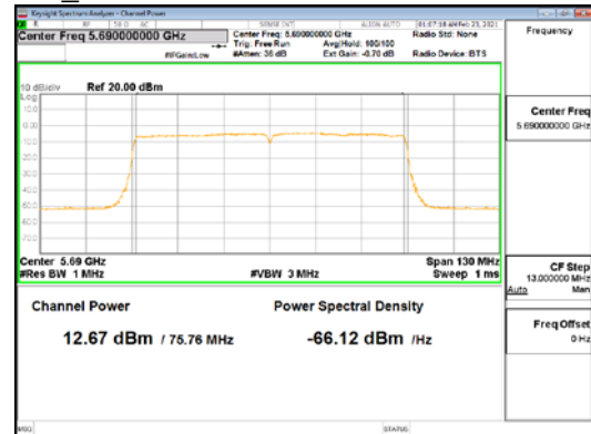
ANT1_802.11ac_VHT80_UNII 2C
