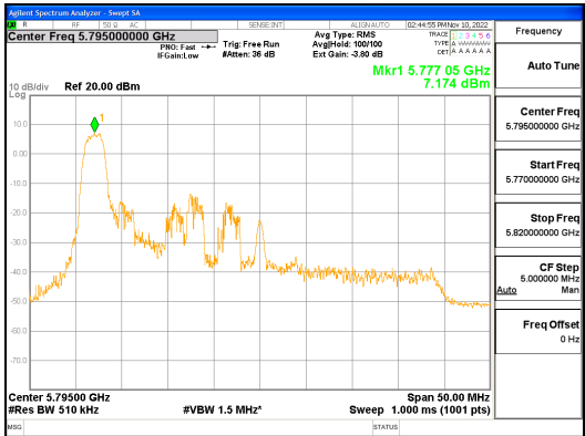
ANT2_802.11ax_HE40_26T_UNII 3
