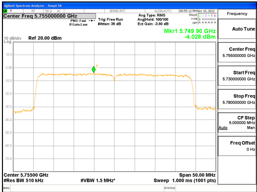
ANT2_802.11ax_HE40_484T_UNII 3
