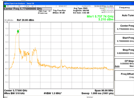
ANT1_802.11ax_HE80_26T_UNII 3
