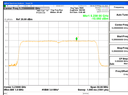
ANT2_802.11ax_HE40_484T_UNII 1
