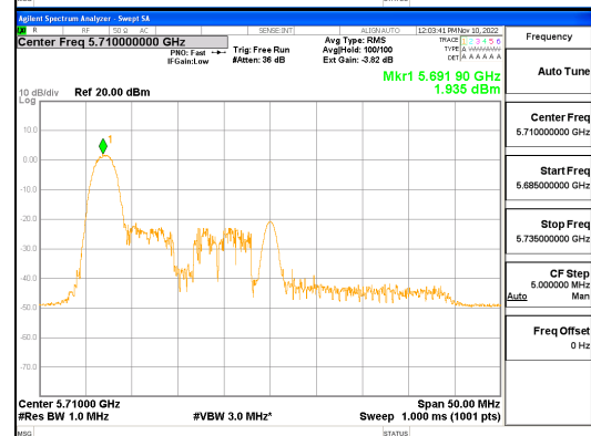
ANT1_802.11ax_HE40_26T_UNII 2C
