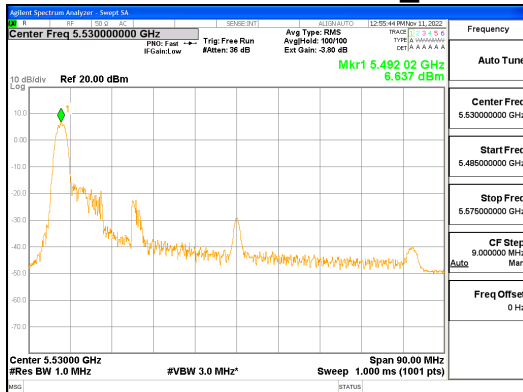
ANT2_802.11ax_HE80_26T_UNII 2C
