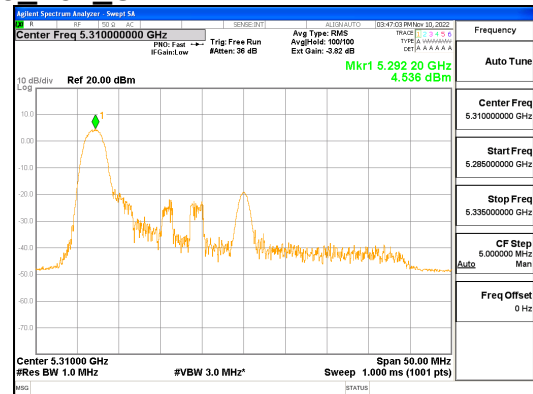
ANT1_802.11ax_HE40_26T_UNII 2A
