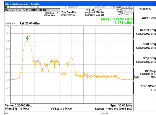
ANT1_802.11ax_HE40_26T_UNII 1
