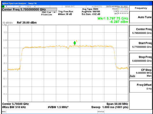
ANT1_802.11ax_HE40_484T_UNII 3
