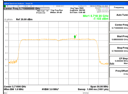
ANT2_802.11ax_HE40_484T_UNII 2C
