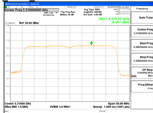
ANT2_802.11ax_HE40_484T_UNII 2A
