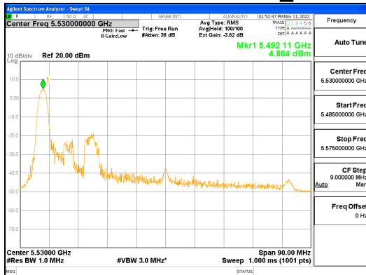
ANT1_802.11ax_HE80_26T_UNII 2C
