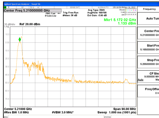
ANT2_802.11ax_HE80_26T_UNII 1
