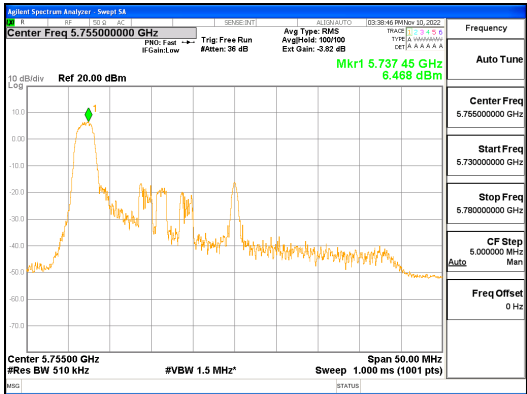
ANT1_802.11ax_HE40_26T_UNII 3
