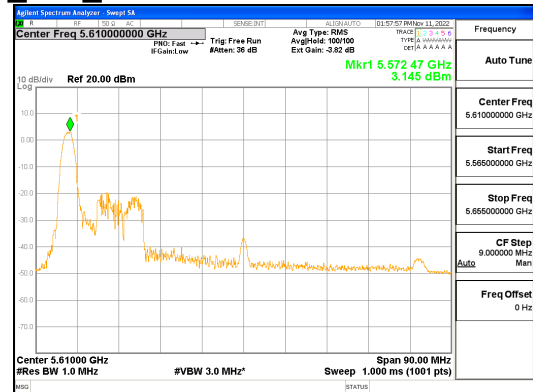
ANT1_802.11ax_HE80_26T_UNII 2C
