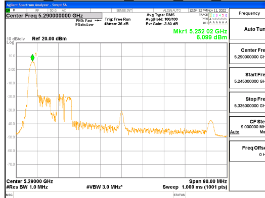
ANT2_802.11ax_HE80_26T_UNII 2A
