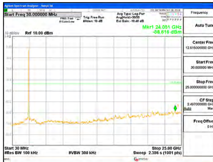
802.11n_HT40_ANT2
