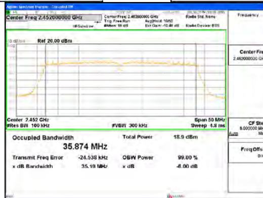
802.11n_HT40_ANT2
