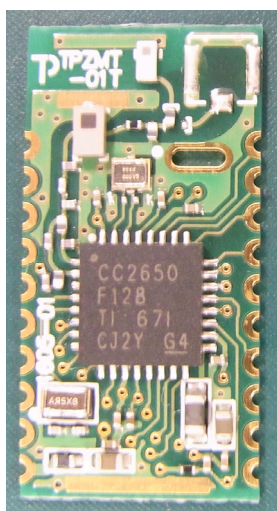
Top (without shield)
