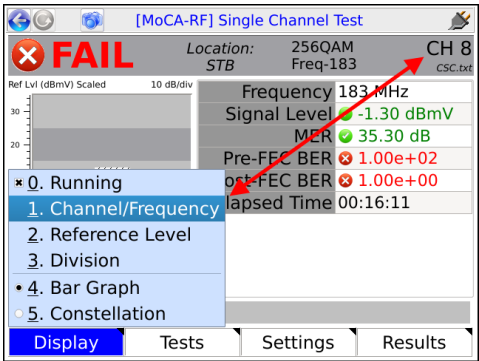
Figure 8-5 Display menu
