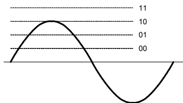
Figure 8-11 Hypothetical RF waveform representing a binary 10 (decimal 3)
