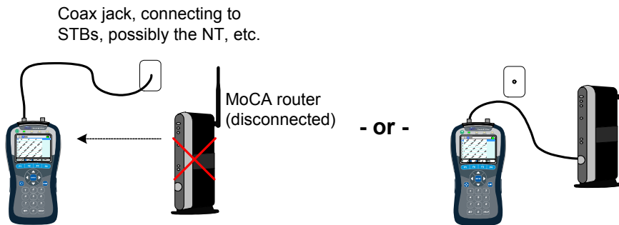
Figure 7-6 Emulating a router - Possible connection setups
