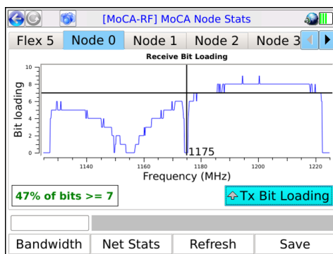
Figure 7-11 Bit-loading graph
