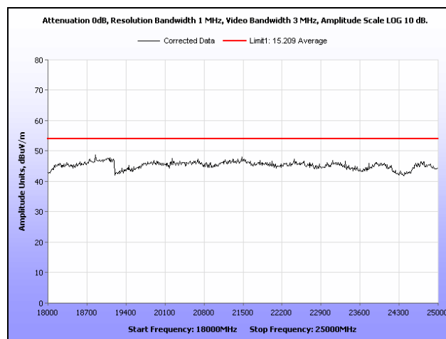
Plot 117. Radiated Spurious Emissions, High Channel, 18 GHz – 25 GHz, Peak under Average, Radio 3
