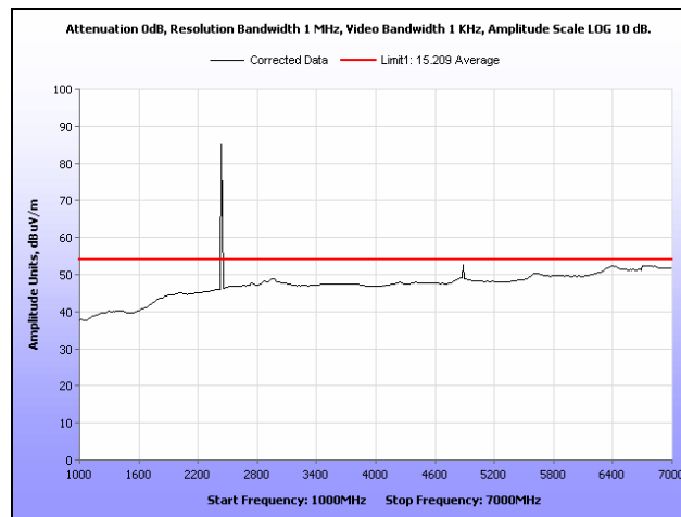
Plot 107. Radiated Spurious Emissions, Mid Channel 1 GHz – 7 GHz, Average, Radio 3
