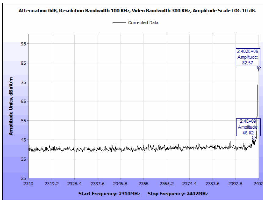
Plot 199. Band Edge 247(d), Radio 2, Low Channel
