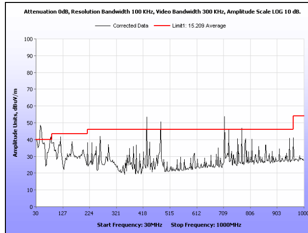
Plot 179. RF Spurious Emissions, Low Channel, 30 MHz – 1 GHz, Radio 4
