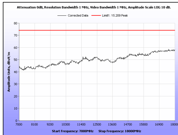
Plot 80. Radiated Spurious Emissions, High Channel, 7 GHz – 18 GHz, Peak, Radio 1
