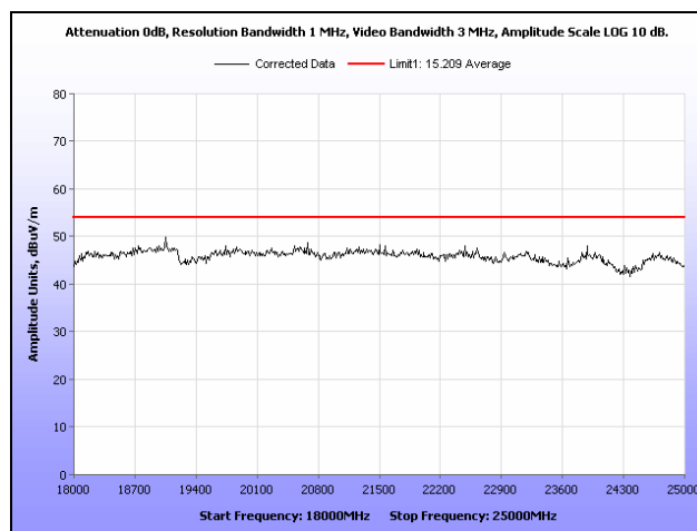
Plot 87. Radiated Spurious Emissions, Low Channel, 18 GHz – 25 GHz, Peak under Average, Radio 2
