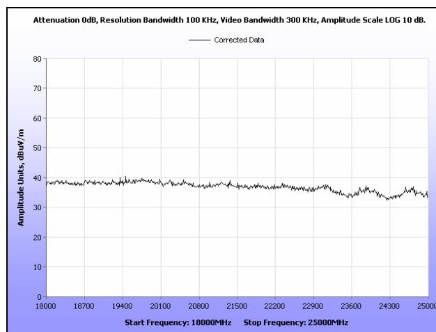
Plot 178. RF Spurious Emissions, High Channel, 18 GHz – 25 GHz, Radio 3
