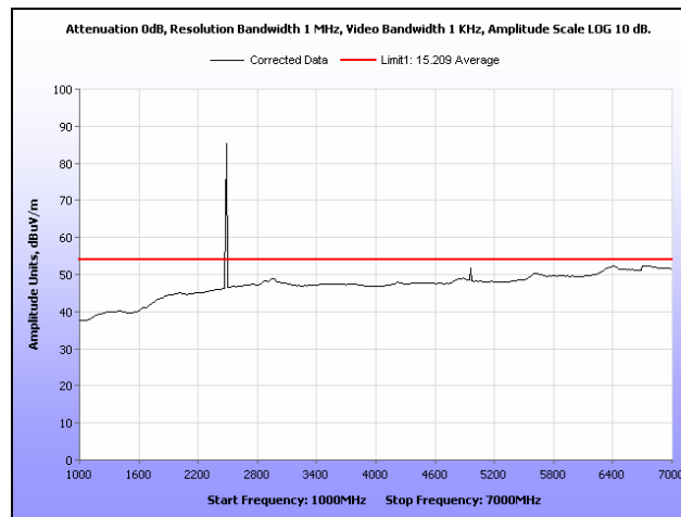
Plot 113. Radiated Spurious Emissions, High Channel, 1 GHz – 7 GHz, Average, Radio 3
