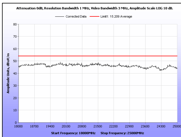
Plot 99. Radiated Spurious Emissions, High Channel, 18 GHz – 25 GHz, Peak under Average, Radio 2
