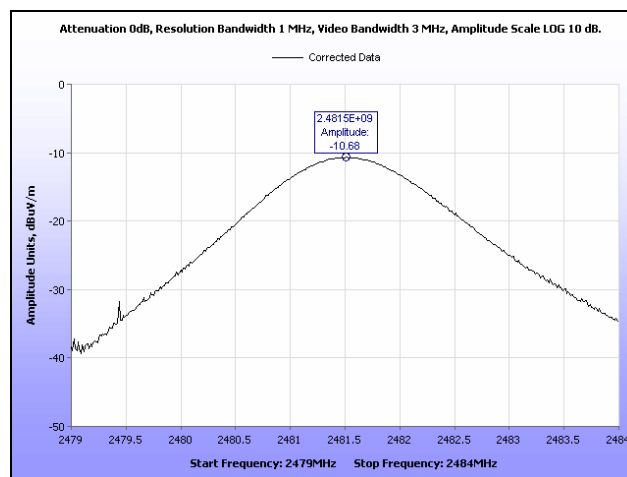
Plot 59. Peak Power Output, High Channel, EIRP, Radio 3
