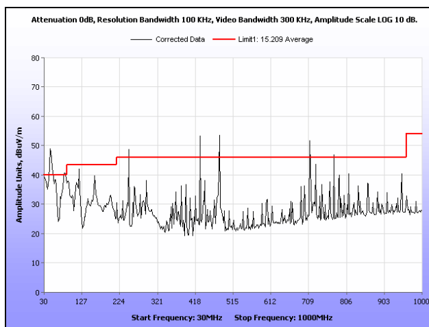
Plot 163. RF Spurious Emissions, High Channel, 30 MHz – 1 GHz, Radio 2
