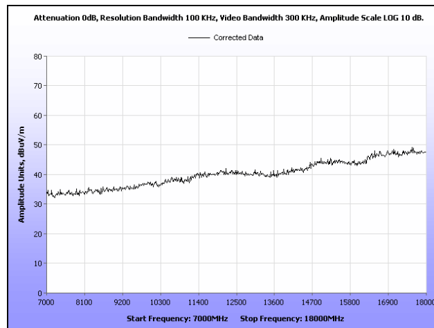
Plot 157. RF Spurious Emissions, Low Channel, 7 GHz – 18 GHz, Radio 2
