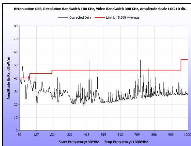
Plot 175. RF Spurious Emissions, High Channel, 30 MHz – 1 GHz, Radio 3
