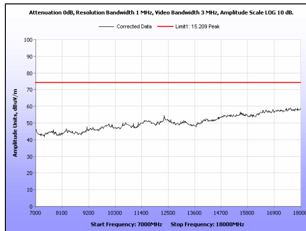
Plot 140. Simultaneous Transmission, 7 GHz – 18 GHz, Peak
