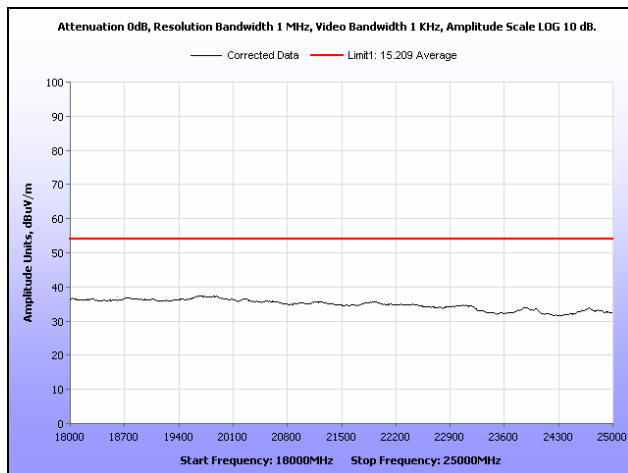
Plot 141. Simultaneous Transmission, 18 GHz – 25 GHz, Average
