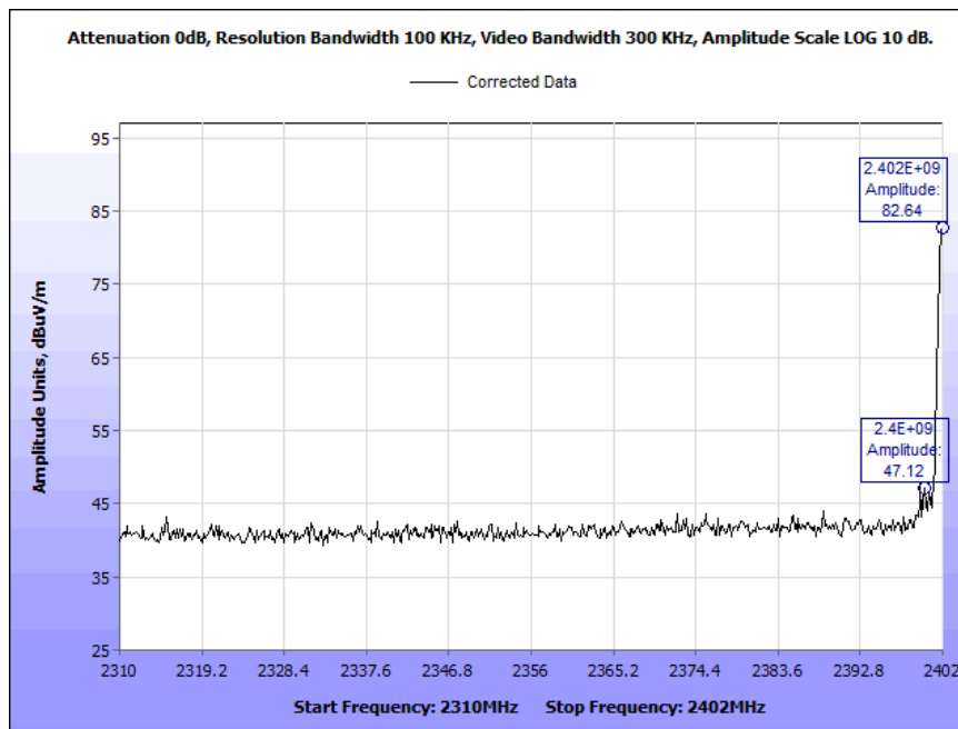
Plot 193. Band Edge 247(d), Radio 1, Low Channel
