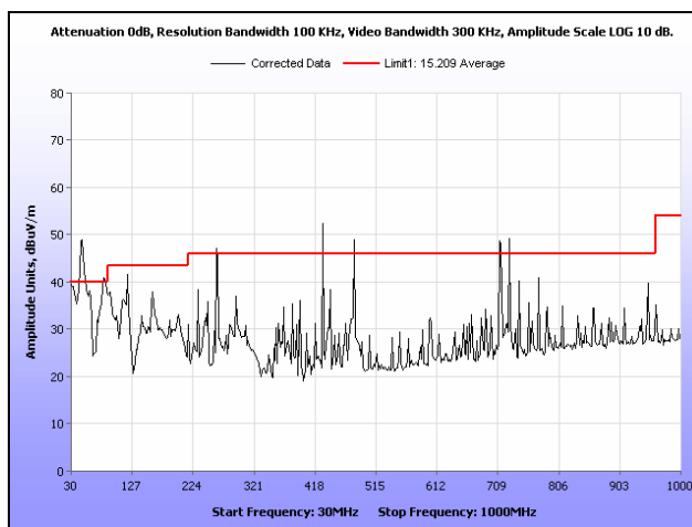
Plot 187. RF Spurious Emissions, High Channel, 30 MHz – 1 GHz, Radio 4
