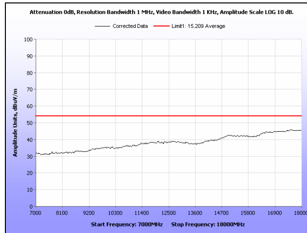
Plot 139. Simultaneous Transmission, 7 GHz – 18 GHz, Average
