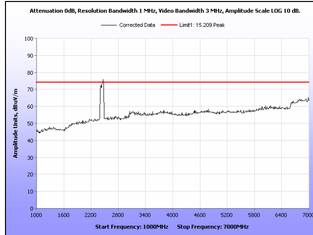
Plot 138. Simultaneous Transmission, 1 GHz – 7 GHz, Peak
