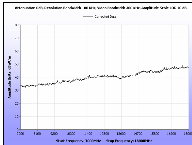
Plot 181. RF Spurious Emissions, Low Channel, 7 GHz – 18 GHz, Radio 4
