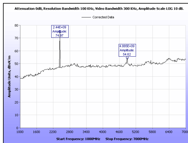
Plot 148. RF Spurious Emissions, Mid Channel, 1 GHz – 7 GHz, Radio 1
