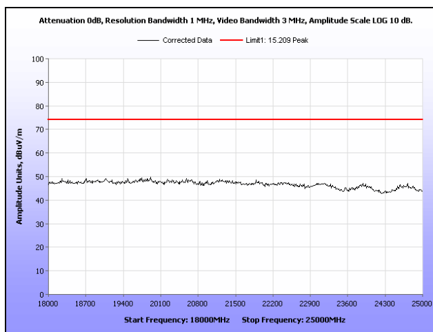
Plot 142. Simultaneous Transmission, 18 GHz – 25 GHz, Peak
