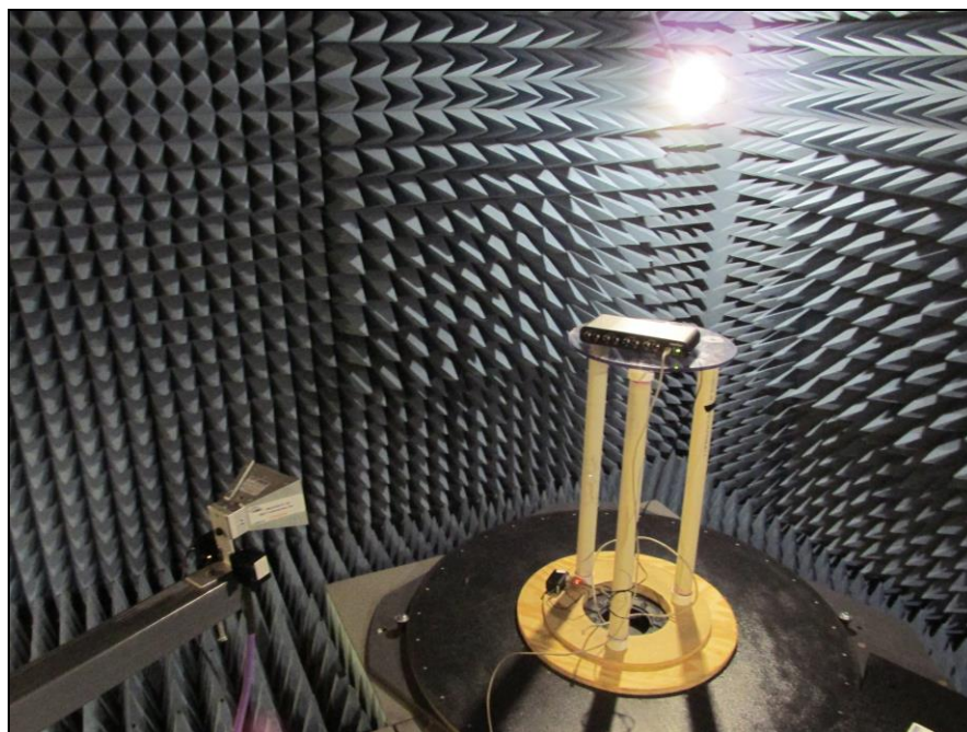
Photograph 8. Radiated Spurious Emissions, Test Setup, 18 GHz – 25 GHz
