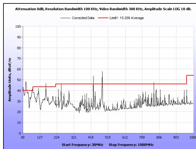
Plot 151. RF Spurious Emissions, High Channel, 30 MHz – 1 GHz, Radio 1
