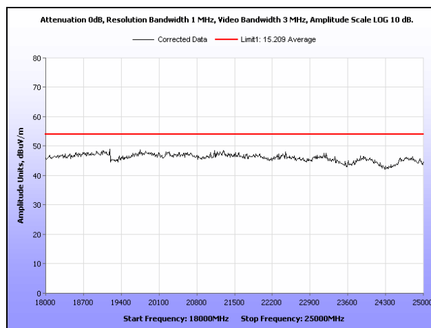
Plot 123. Radiated Spurious Emissions, Low Channel, 18 GHz – 25 GHz, Peak under Average, Radio 4
