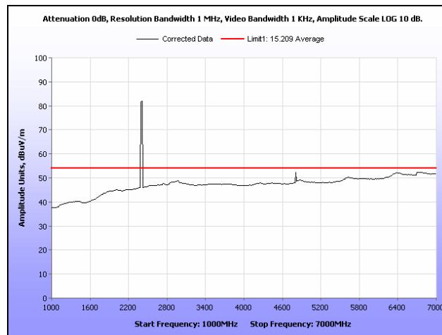
Plot 101. Radiated Spurious Emissions, Low Channel, 1 GHz – 7 GHz, Average, Radio 3
