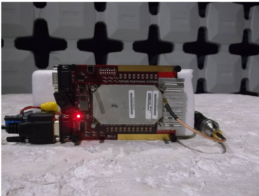
Radiated emissions - EUT Side
