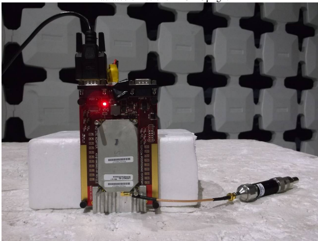
Radiated emissions - EUT Upright
