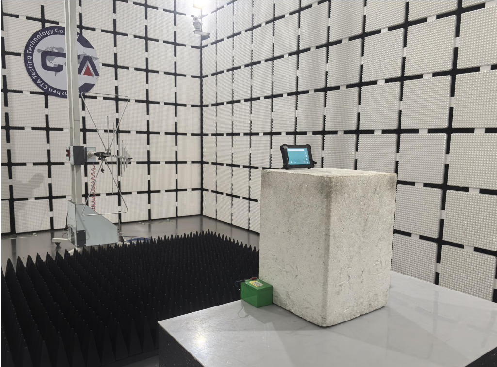
Radiated Emissions Measurement (Below 1GHz)
