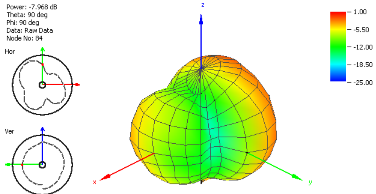
Radiation Pattern at 850 MHz.
