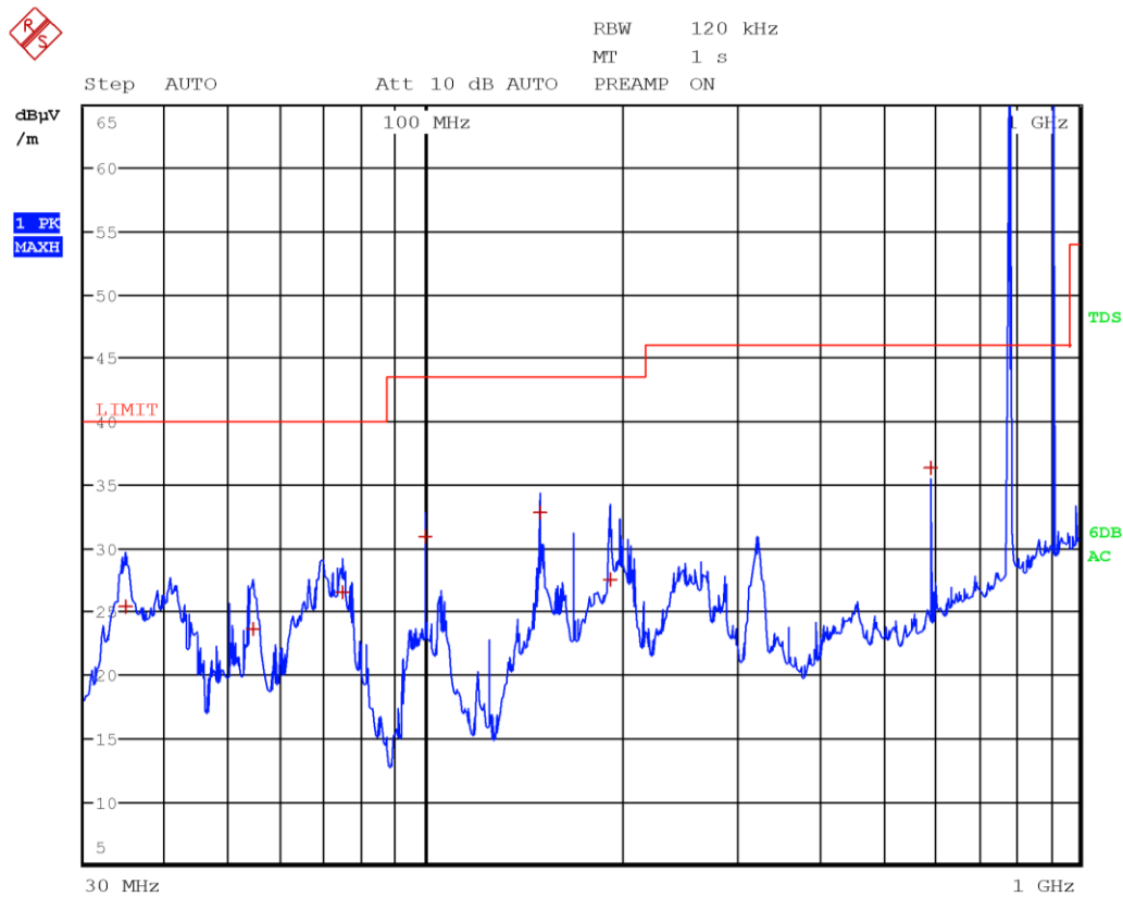
Radiated spurious emissions with antenna in vertical polarization and with LTE Tx at 782 MHz, UHF Tx at 915 MHz, WIFI Tx at 2437 MHz and BT Tx at 2441 MHz (antenna configuration 1)
