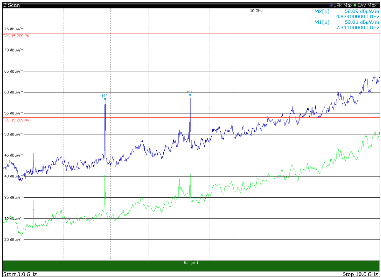
Radiated spurious emissions with antenna in horizontal polarization and with LTE Tx at 1732.5 MHz, UHF Tx at 915 MHz, WIFI Tx at 2437 MHz and BT Tx at 2441 MHz (antenna configuration 1)
