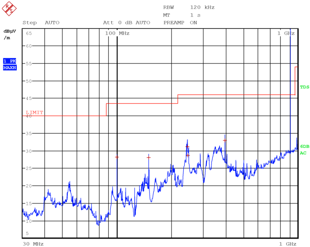
Radiated spurious emissions with antenna in horizontal polarization and with LTE Tx at 1732.5 MHz, UHF Tx at 915 MHz, WIFI Tx at 5220 MHz and BT Tx at 2441 MHz (antenna configuration 1)
