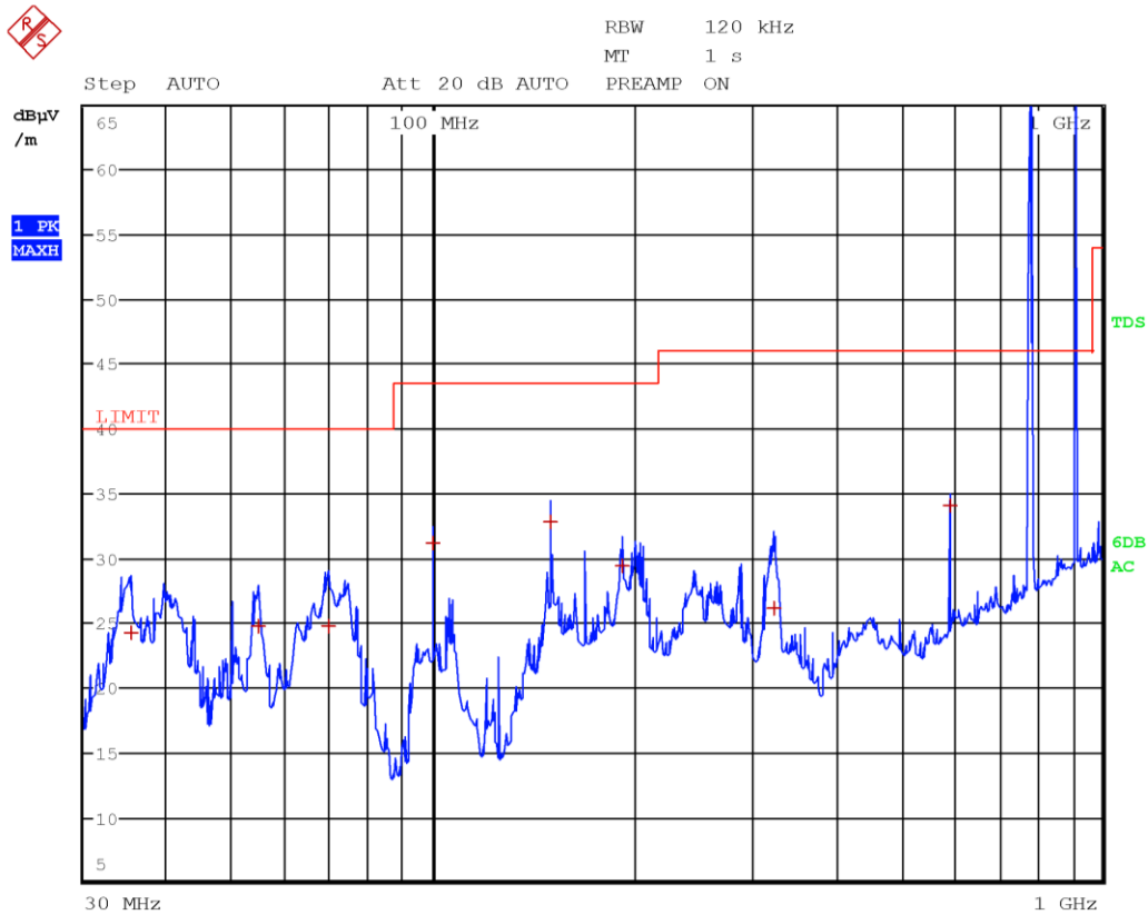
Radiated spurious emissions with antenna in vertical polarization and with LTE Tx at 782 MHz, UHF Tx at 915 MHz, WIFI Tx at 5220 MHz and BT Tx at 2441 MHz (antenna configuration 1)
