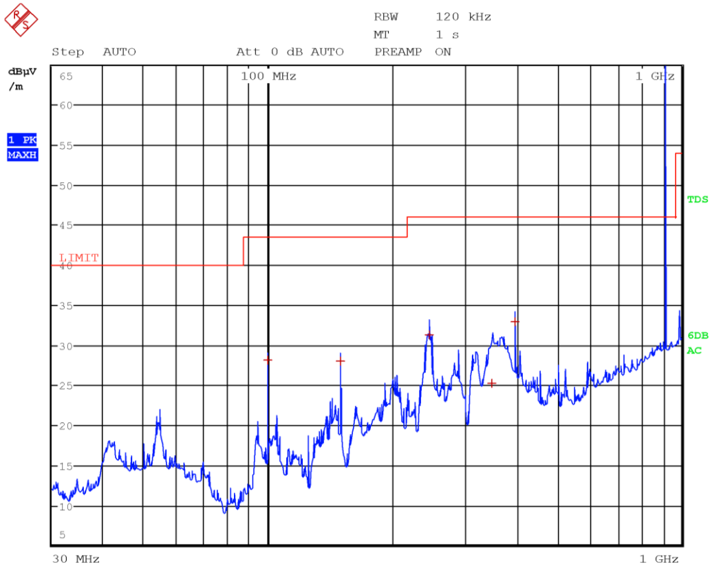
Radiated spurious emissions with antenna in horizontal polarization and with LTE Tx at 1732.5 MHz, UHF Tx at 915 MHz, WIFI Tx at 2437 MHz and BT Tx at 2441 MHz (antenna configuration 1)
